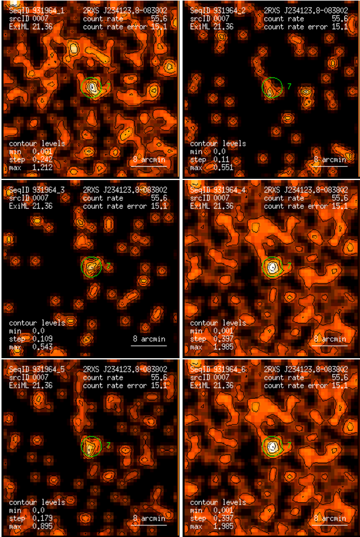
Figure 7: RASS 931964: detection 0007: band rate images, Gaussian filter: (1) PSPC channels 11 – 41, (2) 52 – 90, (3) 91 – 201, (4) 11 – 235, (5) 52 – 201, (6) 11 – 201. Broad band rates in counts/ks. Band rate contour levels in counts/ks/arcmin 2 .
