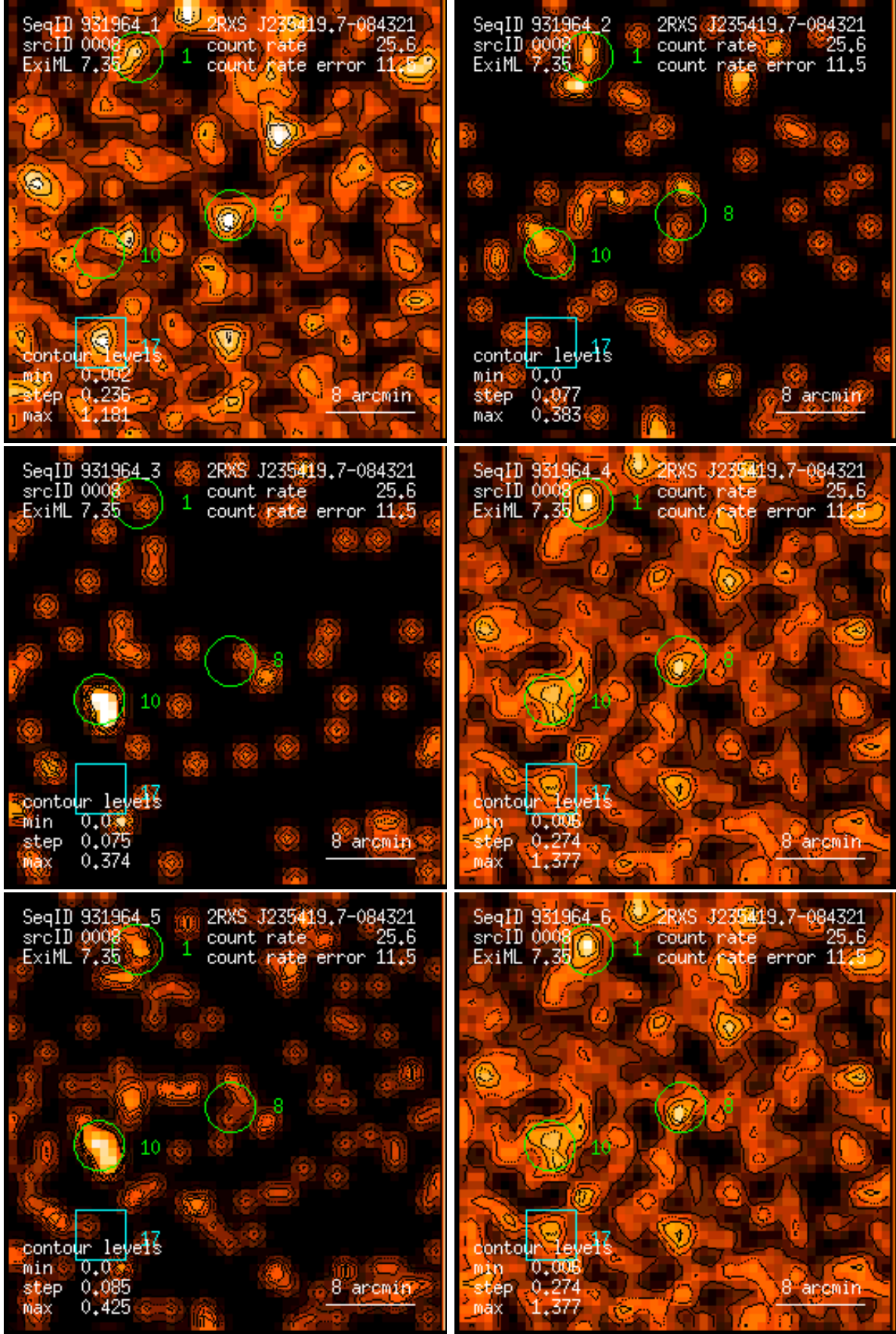
Figure 8: RASS 931964: detection 0008: band rate images, Gaussian filter: (1) PSPC channels 11 – 41, (2) 52 – 90, (3) 91 – 201, (4) 11 – 235, (5) 52 – 201, (6) 11 – 201. Broad band rates in counts/ks. Band rate contour levels in counts/ks/arcmin 2 .
