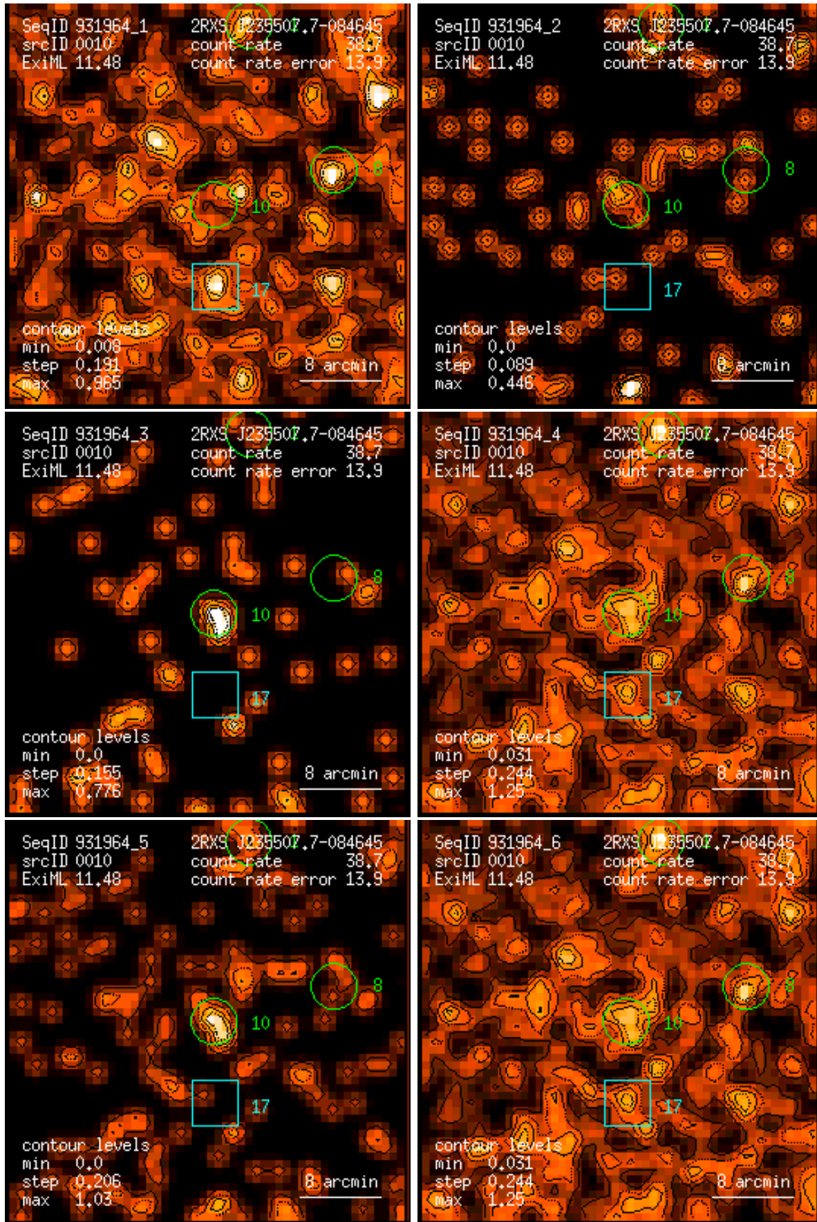
Figure 10: RASS 931964: detection 0010: band rate images, Gaussian filter: (1) PSPC channels 11 – 41, (2) 52 – 90, (3) 91 – 201, (4) 11 – 235, (5) 52 – 201, (6) 11 – 201. Broad band rates in counts/ks. Band rate contour levels in counts/ks/arcmin 2 .
