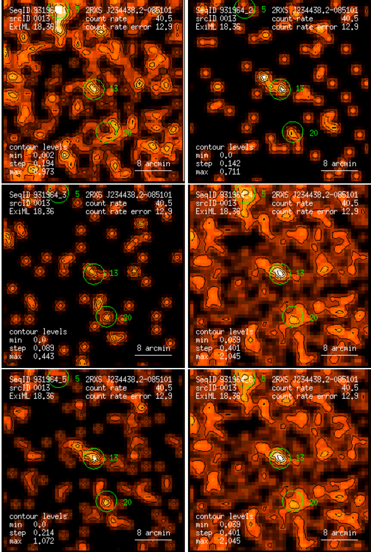
Figure 13: RASS 931964: detection 0013: band rate images, Gaussian filter: (1) PSPC channels 11 – 41, (2) 52 – 90, (3) 91 – 201, (4) 11 – 235, (5) 52 – 201, (6) 11 – 201. Broad band rates in counts/ks. Band rate contour levels in counts/ks/arcmin 2 .
