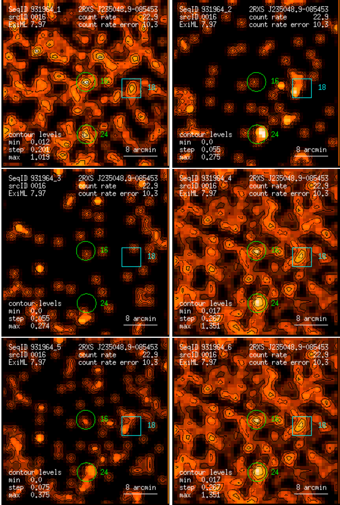
Figure 16: RASS 931964: detection 0016: band rate images, Gaussian filter: (1) PSPC channels 11 – 41, (2) 52 – 90, (3) 91 – 201, (4) 11 – 235, (5) 52 – 201, (6) 11 – 201. Broad band rates in counts/ks. Band rate contour levels in counts/ks/arcmin 2 .
