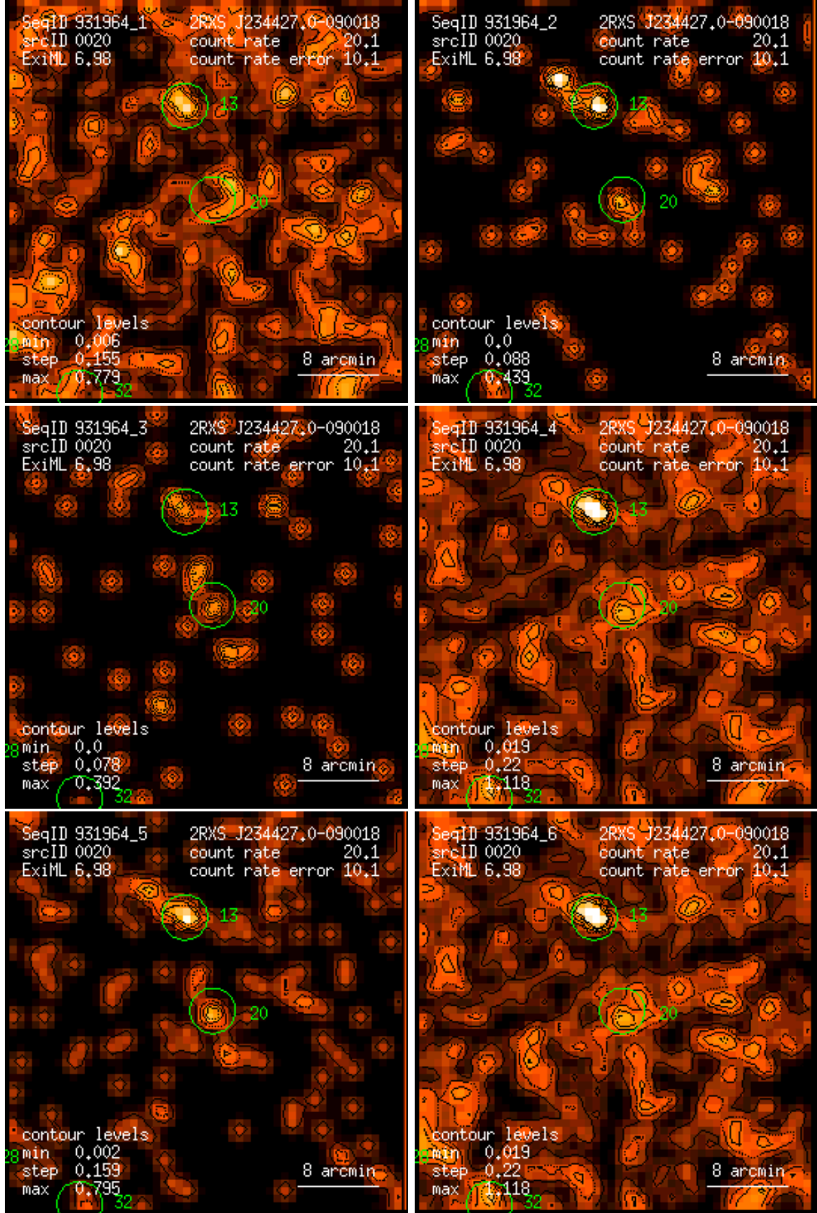
Figure 20: RASS 931964: detection 0020: band rate images, Gaussian filter: (1) PSPC channels 11 – 41, (2) 52 – 90, (3) 91 – 201, (4) 11 – 235, (5) 52 – 201, (6) 11 – 201. Broad band rates in counts/ks. Band rate contour levels in counts/ks/arcmin 2 .
