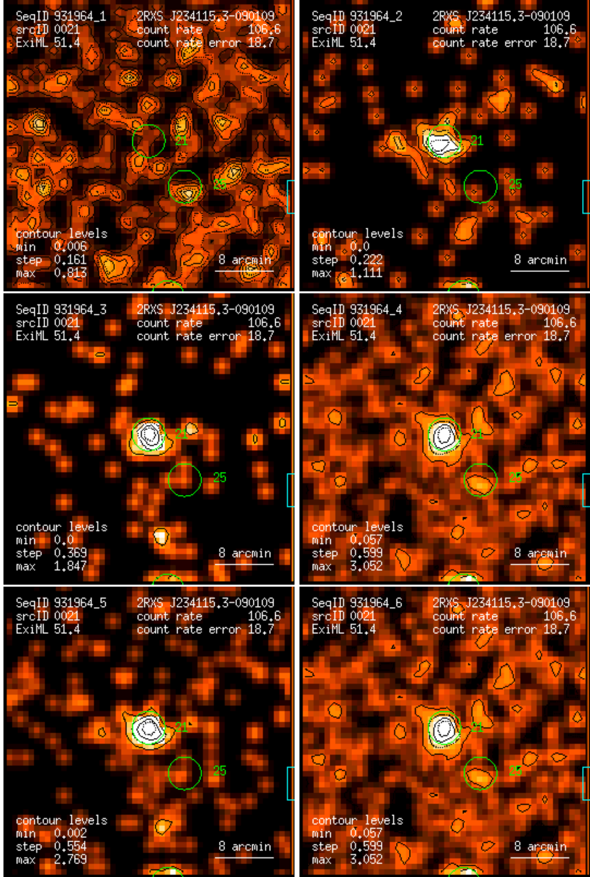
Figure 21: RASS 931964: detection 0021: band rate images, Gaussian filter: (1) PSPC channels 11 – 41, (2) 52 – 90, (3) 91 – 201, (4) 11 – 235, (5) 52 – 201, (6) 11 – 201. Broad band rates in counts/ks. Band rate contour levels in counts/ks/arcmin 2 .
