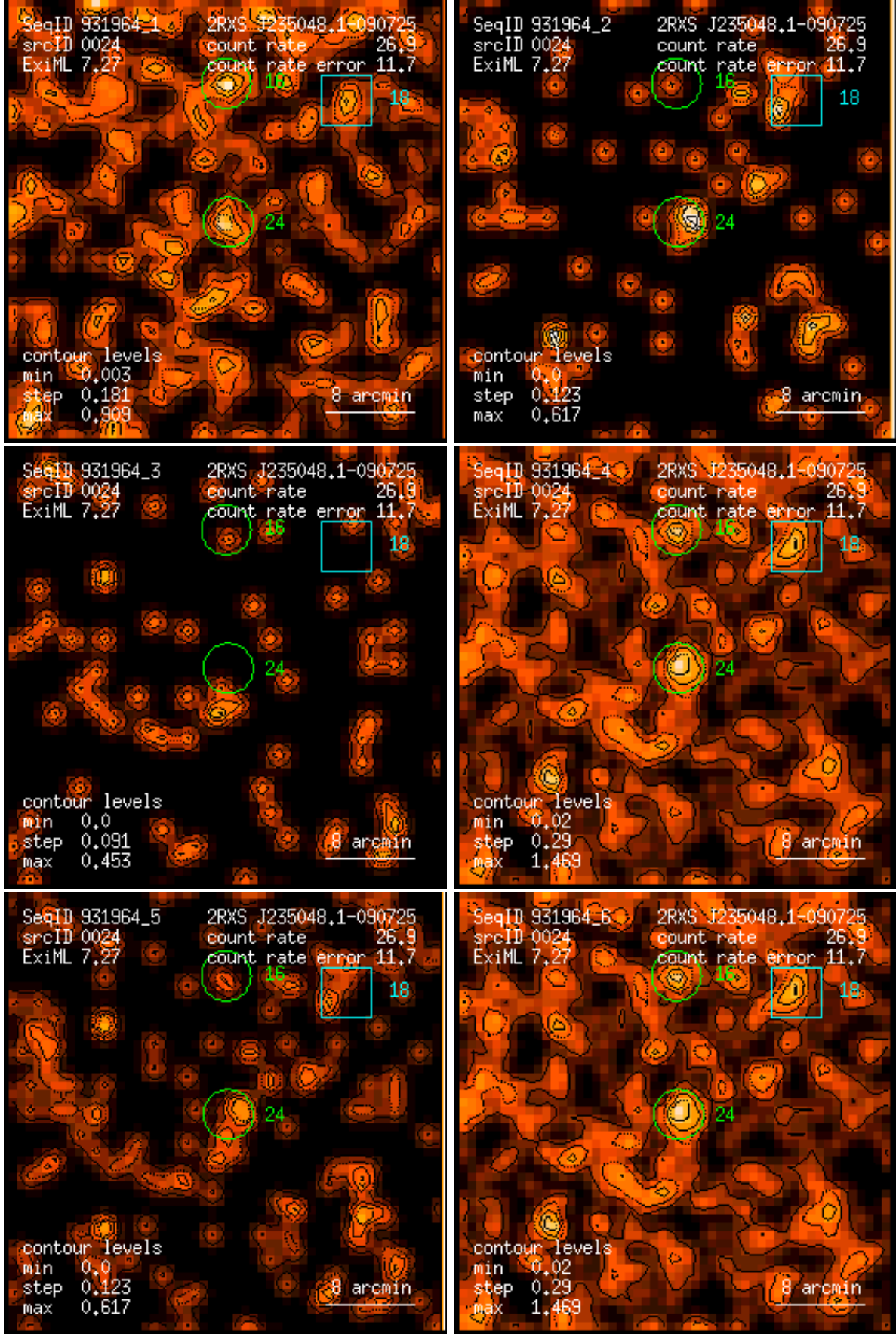
Figure 24: RASS 931964: detection 0024: band rate images, Gaussian filter: (1) PSPC channels 11 – 41, (2) 52 – 90, (3) 91 – 201, (4) 11 – 235, (5) 52 – 201, (6) 11 – 201. Broad band rates in counts/ks. Band rate contour levels in counts/ks/arcmin 2 .
