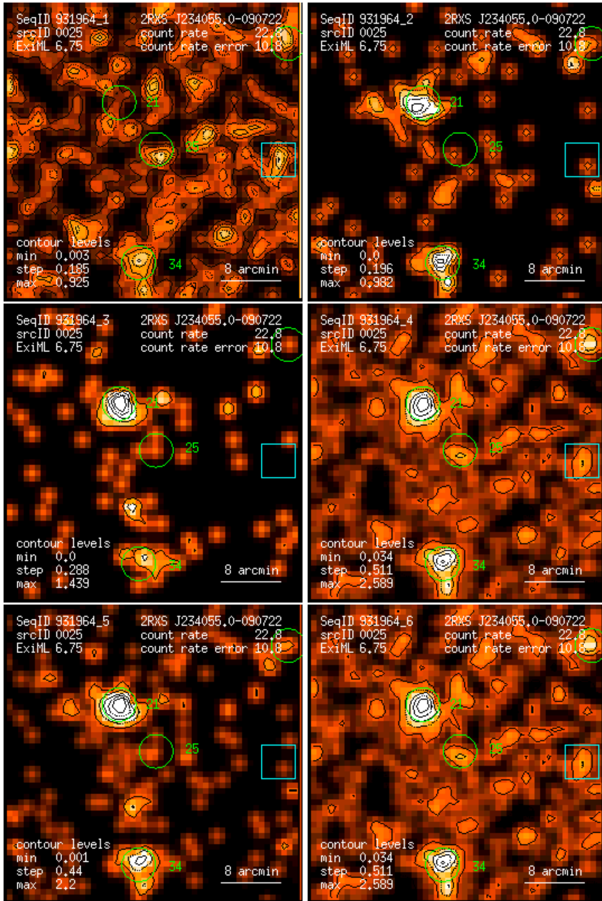
Figure 25: RASS 931964: detection 0025: band rate images, Gaussian filter: (1) PSPC channels 11 – 41, (2) 52 – 90, (3) 91 – 201, (4) 11 – 235, (5) 52 – 201, (6) 11 – 201. Broad band rates in counts/ks. Band rate contour levels in counts/ks/arcmin 2 .
