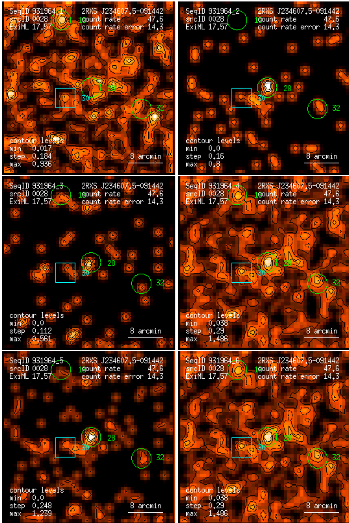
Figure 28: RASS 931964: detection 0028: band rate images, Gaussian filter: (1) PSPC channels 11 – 41, (2) 52 – 90, (3) 91 – 201, (4) 11 – 235, (5) 52 – 201, (6) 11 – 201. Broad band rates in counts/ks. Band rate contour levels in counts/ks/arcmin 2 .
