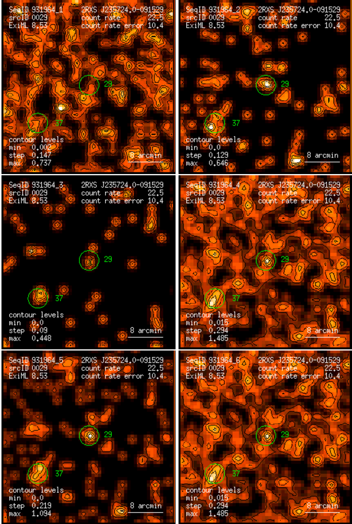
Figure 29: RASS 931964: detection 0029: band rate images, Gaussian filter: (1) PSPC channels 11 – 41, (2) 52 – 90, (3) 91 – 201, (4) 11 – 235, (5) 52 – 201, (6) 11 – 201. Broad band rates in counts/ks. Band rate contour levels in counts/ks/arcmin 2 .
