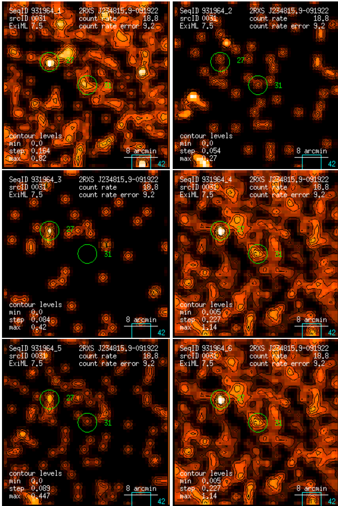
Figure 31: RASS 931964: detection 0031: band rate images, Gaussian filter: (1) PSPC channels 11 – 41, (2) 52 – 90, (3) 91 – 201, (4) 11 – 235, (5) 52 – 201, (6) 11 – 201. Broad band rates in counts/ks. Band rate contour levels in counts/ks/arcmin 2 .
