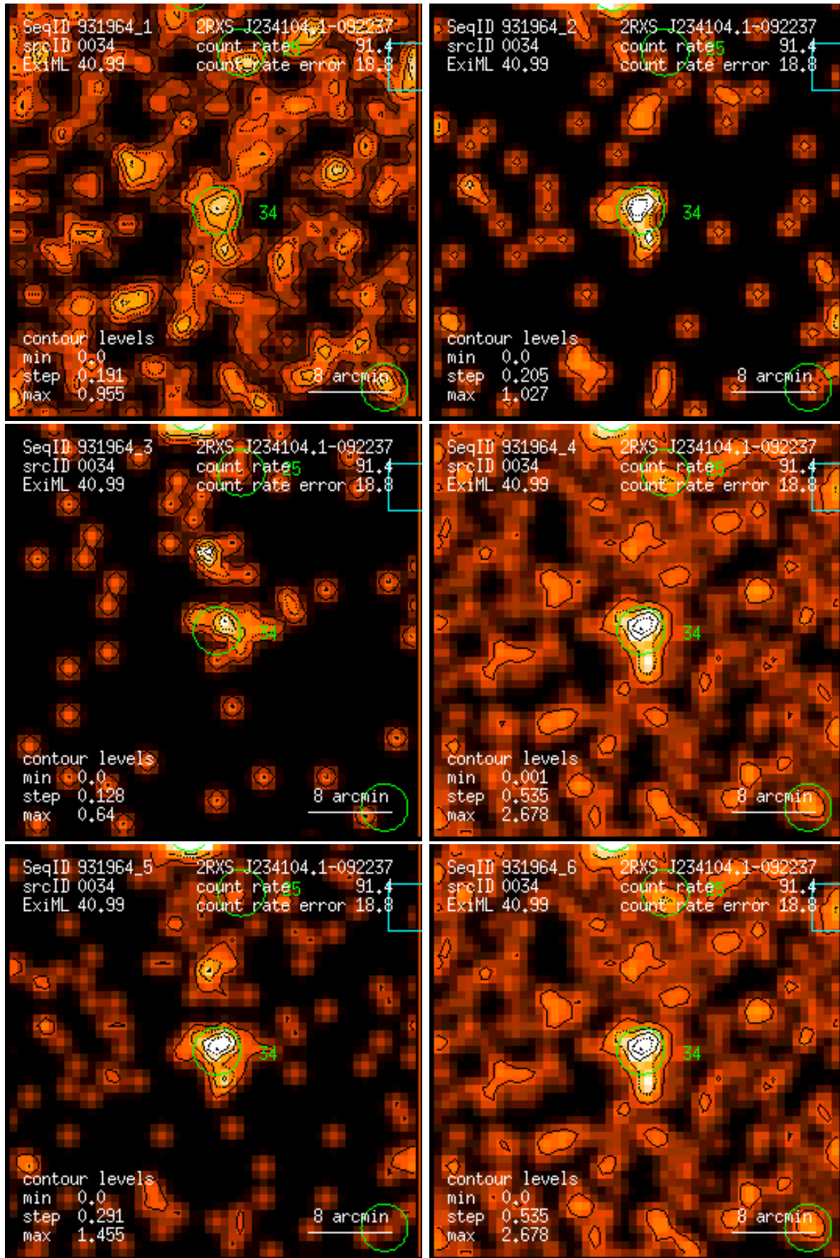
Figure 34: RASS 931964: detection 0034: band rate images, Gaussian filter: (1) PSPC channels 11 – 41, (2) 52 – 90, (3) 91 – 201, (4) 11 – 235, (5) 52 – 201, (6) 11 – 201. Broad band rates in counts/ks. Band rate contour levels in counts/ks/arcmin 2 .
