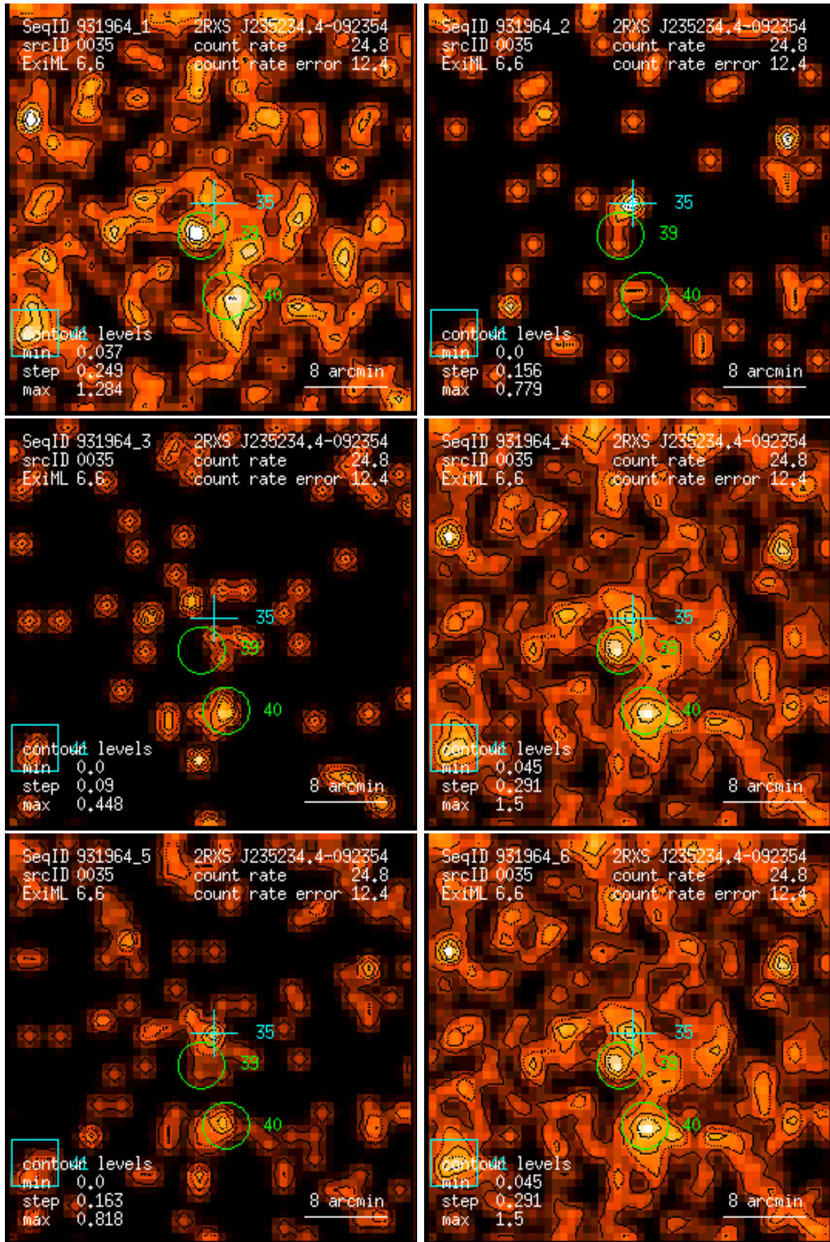
Figure 35: RASS 931964: detection 0035: band rate images, Gaussian filter: (1) PSPC channels 11 – 41, (2) 52 – 90, (3) 91 – 201, (4) 11 – 235, (5) 52 – 201, (6) 11 – 201. Broad band rates in counts/ks. Band rate contour levels in counts/ks/arcmin 2 .
