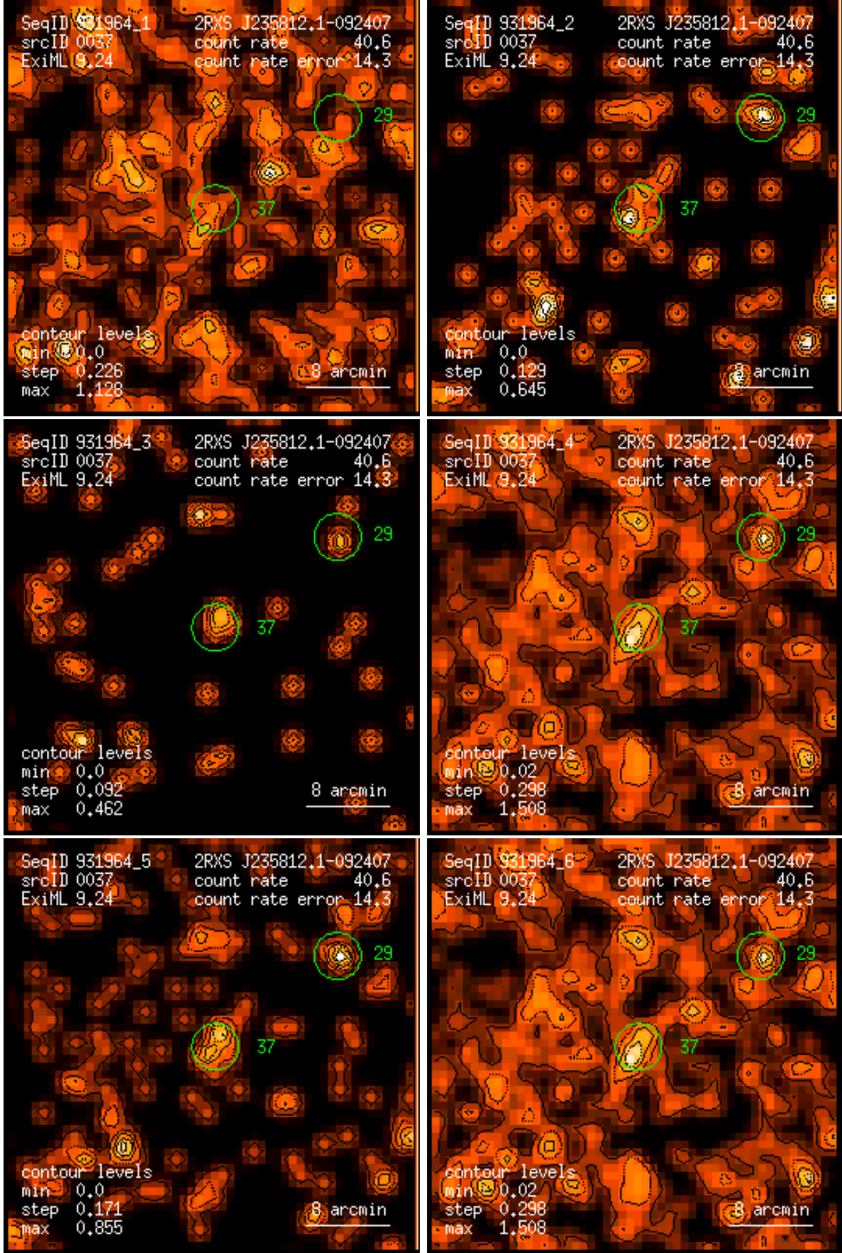
Figure 37: RASS 931964: detection 0037: band rate images, Gaussian filter: (1) PSPC channels 11 – 41, (2) 52 – 90, (3) 91 – 201, (4) 11 – 235, (5) 52 – 201, (6) 11 – 201. Broad band rates in counts/ks. Band rate contour levels in counts/ks/arcmin 2 .
