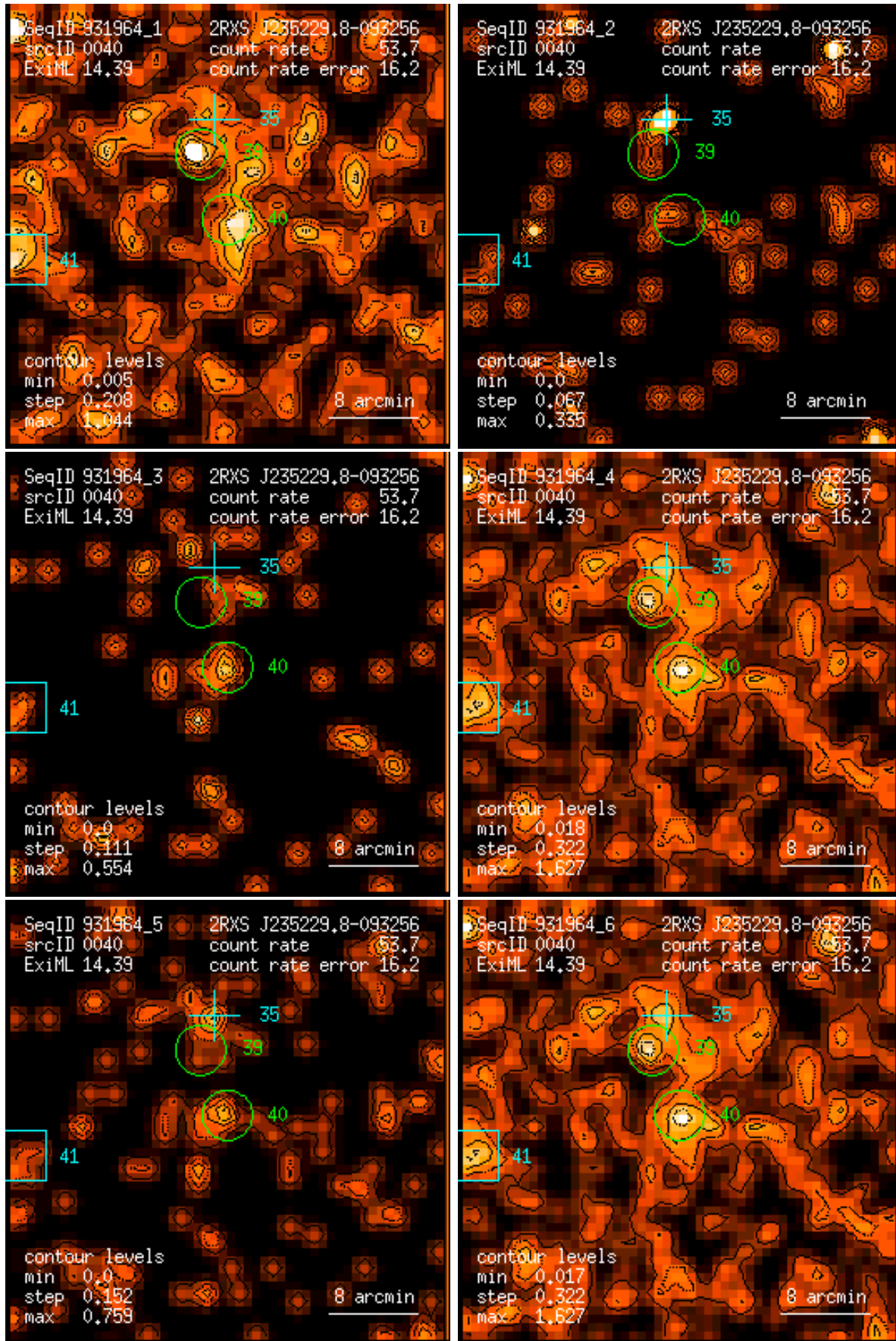
Figure 40: RASS 931964: detection 0040: band rate images, Gaussian filter: (1) PSPC channels 11 – 41, (2) 52 – 90, (3) 91 – 201, (4) 11 – 235, (5) 52 – 201, (6) 11 – 201. Broad band rates in counts/ks. Band rate contour levels in counts/ks/arcmin 2 .
