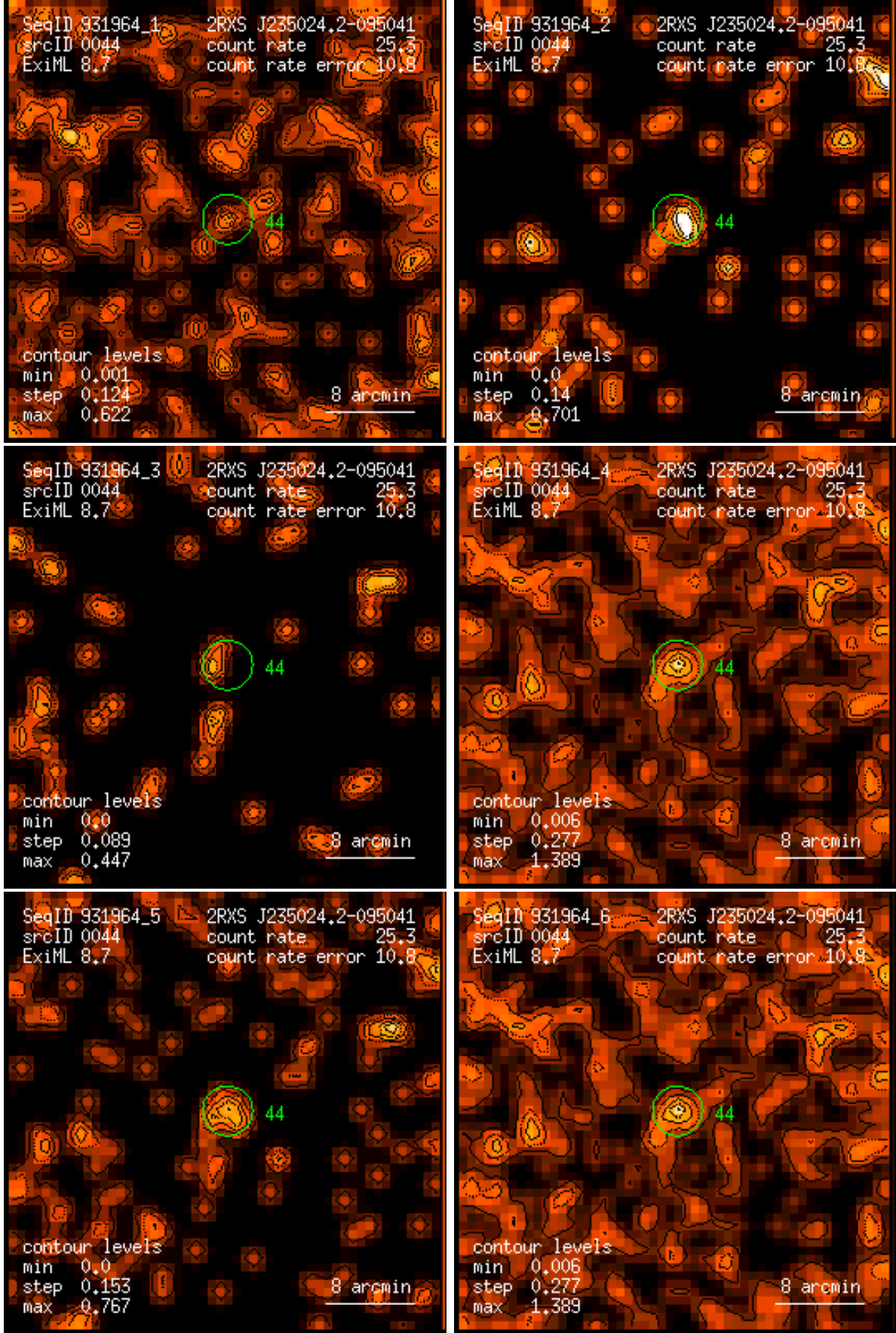
Figure 44: RASS 931964: detection 0044: band rate images, Gaussian filter: (1) PSPC channels 11 – 41, (2) 52 – 90, (3) 91 – 201, (4) 11 – 235, (5) 52 – 201, (6) 11 – 201. Broad band rates in counts/ks. Band rate contour levels in counts/ks/arcmin 2 .
