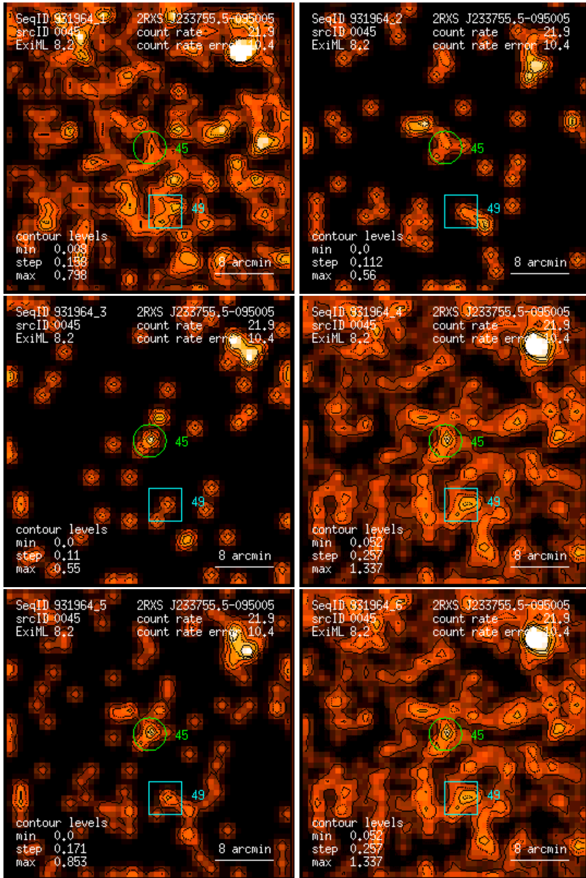
Figure 45: RASS 931964: detection 0045: band rate images, Gaussian filter: (1) PSPC channels 11 – 41, (2) 52 – 90, (3) 91 – 201, (4) 11 – 235, (5) 52 – 201, (6) 11 – 201. Broad band rates in counts/ks. Band rate contour levels in counts/ks/arcmin 2 .
