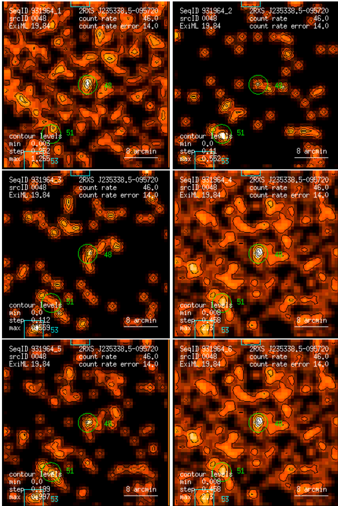
Figure 48: RASS 931964: detection 0048: band rate images, Gaussian filter: (1) PSPC channels 11 – 41, (2) 52 – 90, (3) 91 – 201, (4) 11 – 235, (5) 52 – 201, (6) 11 – 201. Broad band rates in counts/ks. Band rate contour levels in counts/ks/arcmin 2 .
