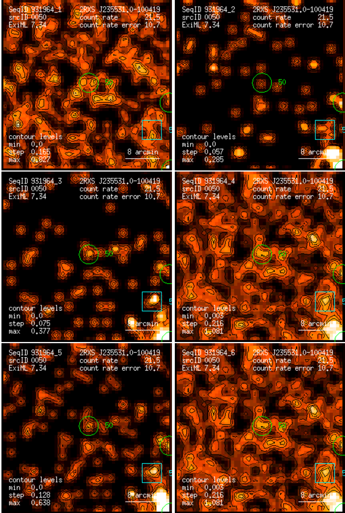
Figure 50: RASS 931964: detection 0050: band rate images, Gaussian filter: (1) PSPC channels 11 – 41, (2) 52 – 90, (3) 91 – 201, (4) 11 – 235, (5) 52 – 201, (6) 11 – 201. Broad band rates in counts/ks. Band rate contour levels in counts/ks/arcmin 2 .
