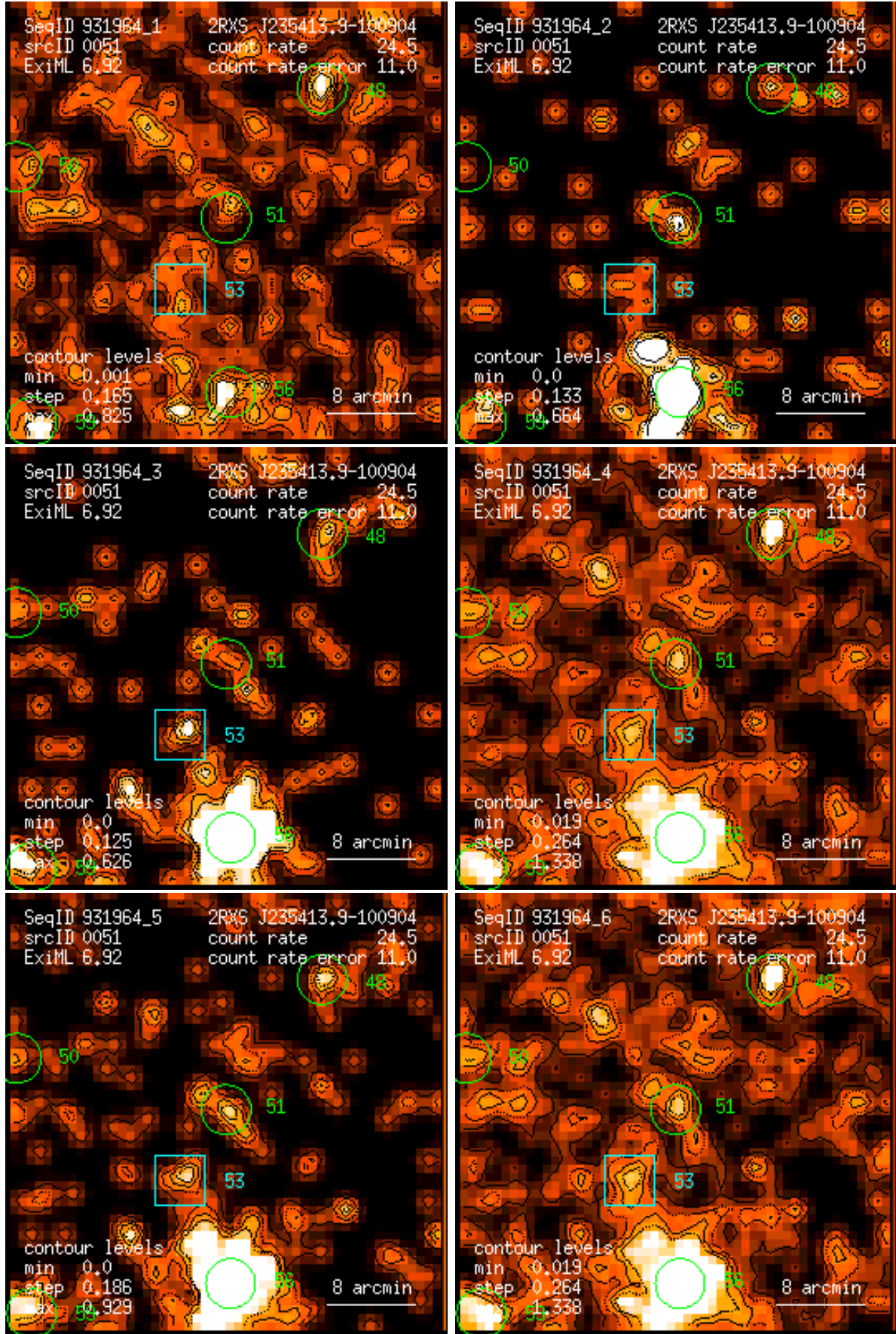
Figure 51: RASS 931964: detection 0051: band rate images, Gaussian filter: (1) PSPC channels 11 – 41, (2) 52 – 90, (3) 91 – 201, (4) 11 – 235, (5) 52 – 201, (6) 11 – 201. Broad band rates in counts/ks. Band rate contour levels in counts/ks/arcmin 2 .
