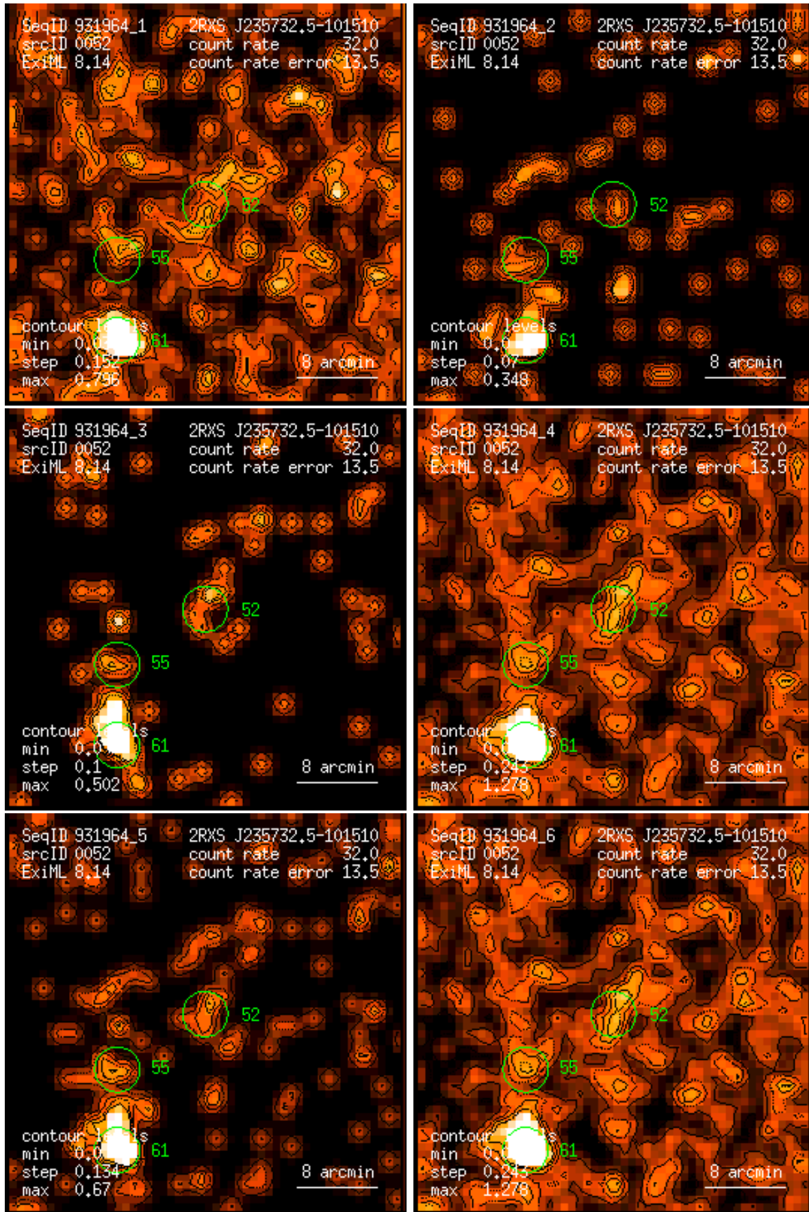
Figure 52: RASS 931964: detection 0052: band rate images, Gaussian filter: (1) PSPC channels 11 – 41, (2) 52 – 90, (3) 91 – 201, (4) 11 – 235, (5) 52 – 201, (6) 11 – 201. Broad band rates in counts/ks. Band rate contour levels in counts/ks/arcmin 2 .
