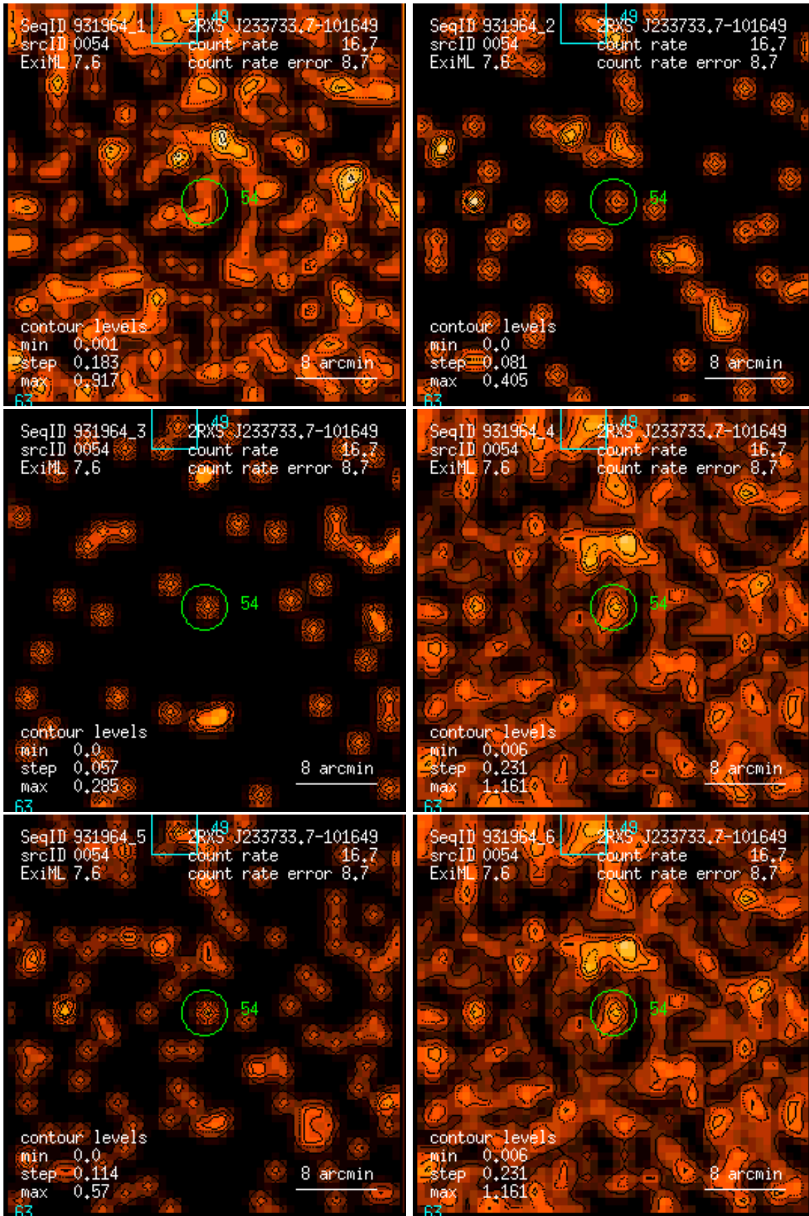
Figure 54: RASS 931964: detection 0054: band rate images, Gaussian filter: (1) PSPC channels 11 – 41, (2) 52 – 90, (3) 91 – 201, (4) 11 – 235, (5) 52 – 201, (6) 11 – 201. Broad band rates in counts/ks. Band rate contour levels in counts/ks/arcmin 2 .
