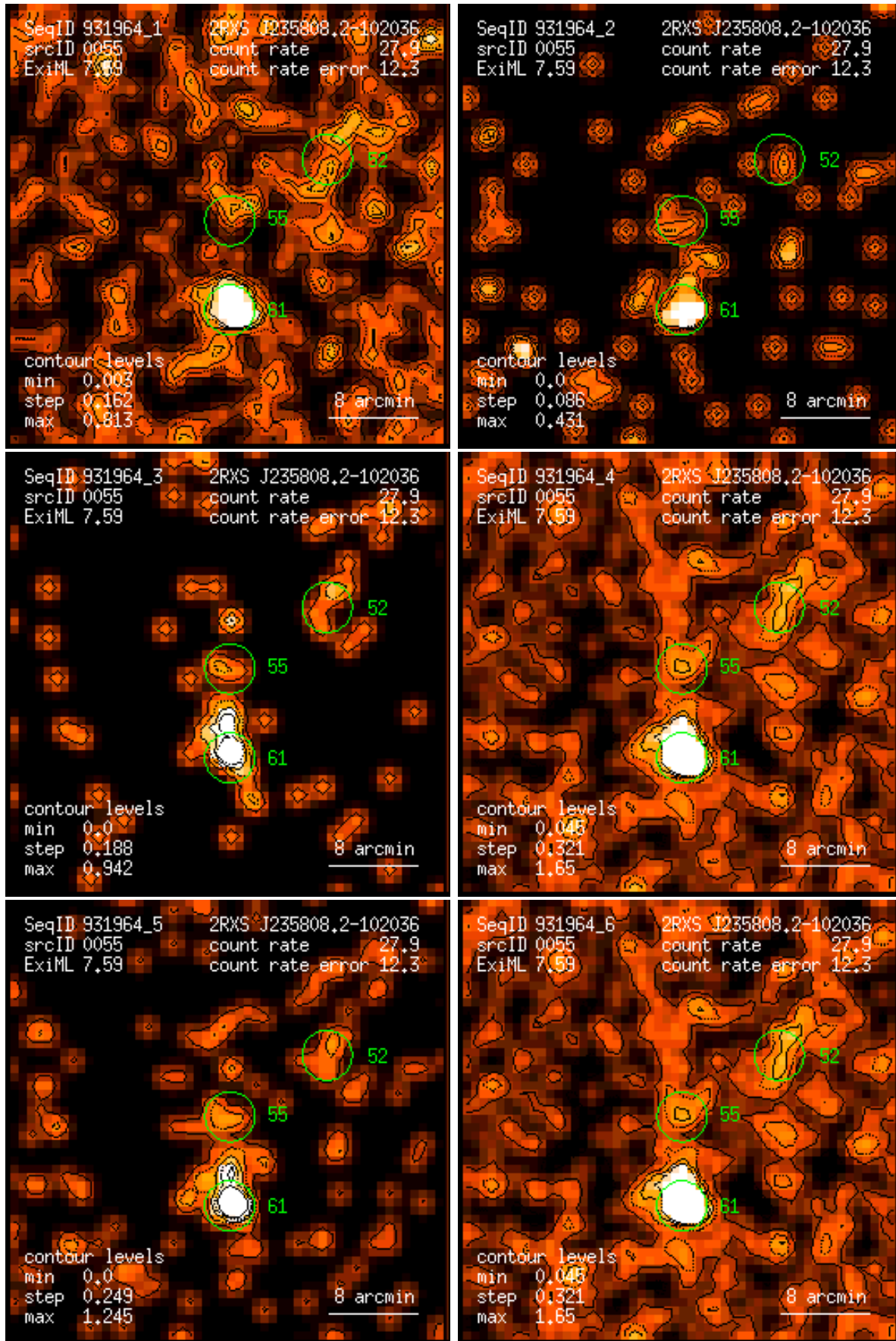
Figure 55: RASS 931964: detection 0055: band rate images, Gaussian filter: (1) PSPC channels 11 – 41, (2) 52 – 90, (3) 91 – 201, (4) 11 – 235, (5) 52 – 201, (6) 11 – 201. Broad band rates in counts/ks. Band rate contour levels in counts/ks/arcmin 2 .
