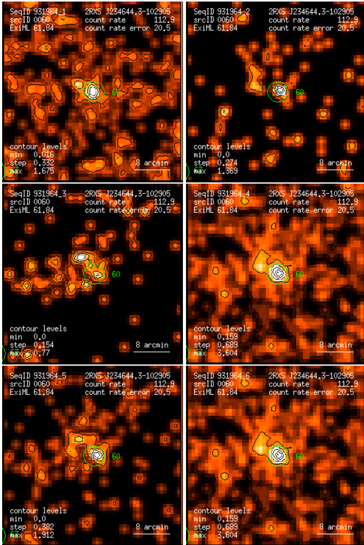
Figure 60: RASS 931964: detection 0060: band rate images, Gaussian filter: (1) PSPC channels 11 – 41, (2) 52 – 90, (3) 91 – 201, (4) 11 – 235, (5) 52 – 201, (6) 11 – 201. Broad band rates in counts/ks. Band rate contour levels in counts/ks/arcmin 2 .
