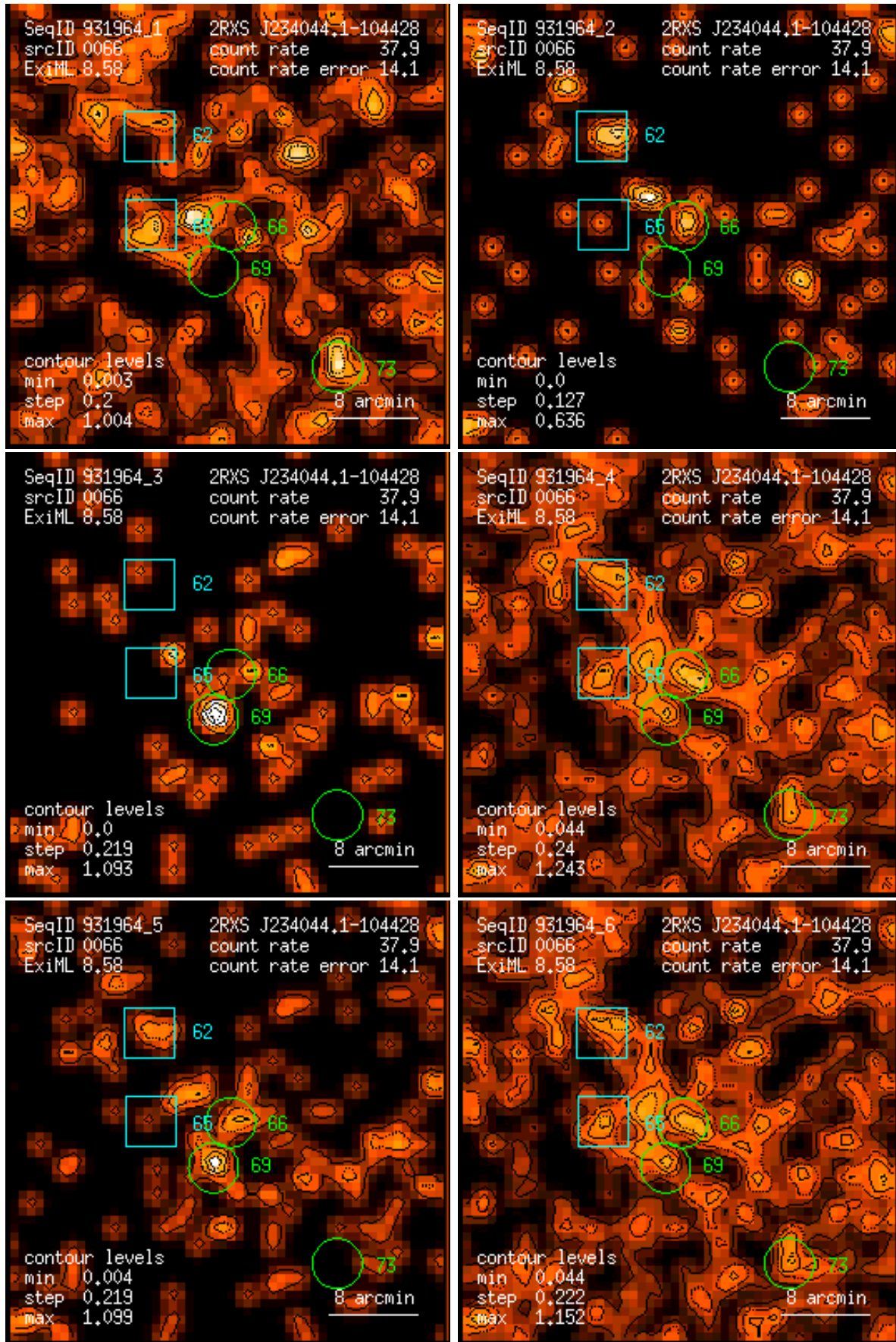
Figure 66: RASS 931964: detection 0066: band rate images, Gaussian filter: (1) PSPC channels 11 – 41, (2) 52 – 90, (3) 91 – 201, (4) 11 – 235, (5) 52 – 201, (6) 11 – 201. Broad band rates in counts/ks. Band rate contour levels in counts/ks/arcmin 2 .
