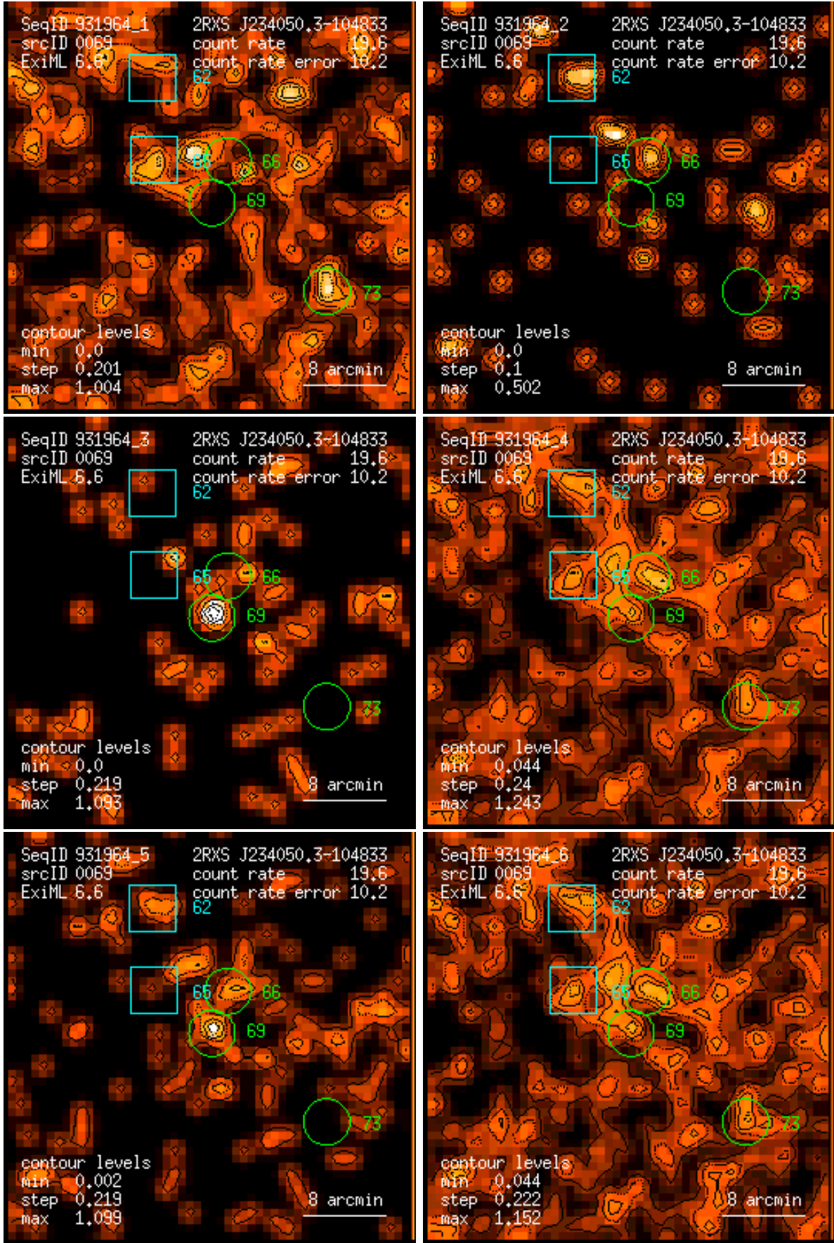
Figure 69: RASS 931964: detection 0069: band rate images, Gaussian filter: (1) PSPC channels 11 – 41, (2) 52 – 90, (3) 91 – 201, (4) 11 – 235, (5) 52 – 201, (6) 11 – 201. Broad band rates in counts/ks. Band rate contour levels in counts/ks/arcmin 2 .
