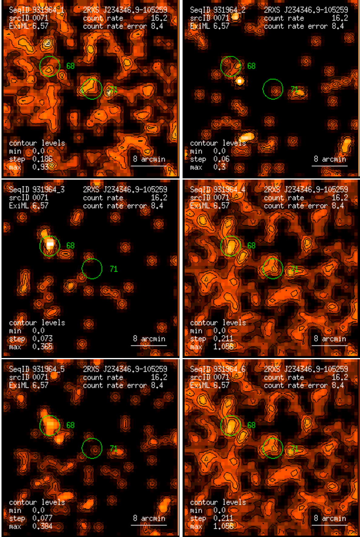
Figure 71: RASS 931964: detection 0071: band rate images, Gaussian filter: (1) PSPC channels 11 – 41, (2) 52 – 90, (3) 91 – 201, (4) 11 – 235, (5) 52 – 201, (6) 11 – 201. Broad band rates in counts/ks. Band rate contour levels in counts/ks/arcmin 2 .
