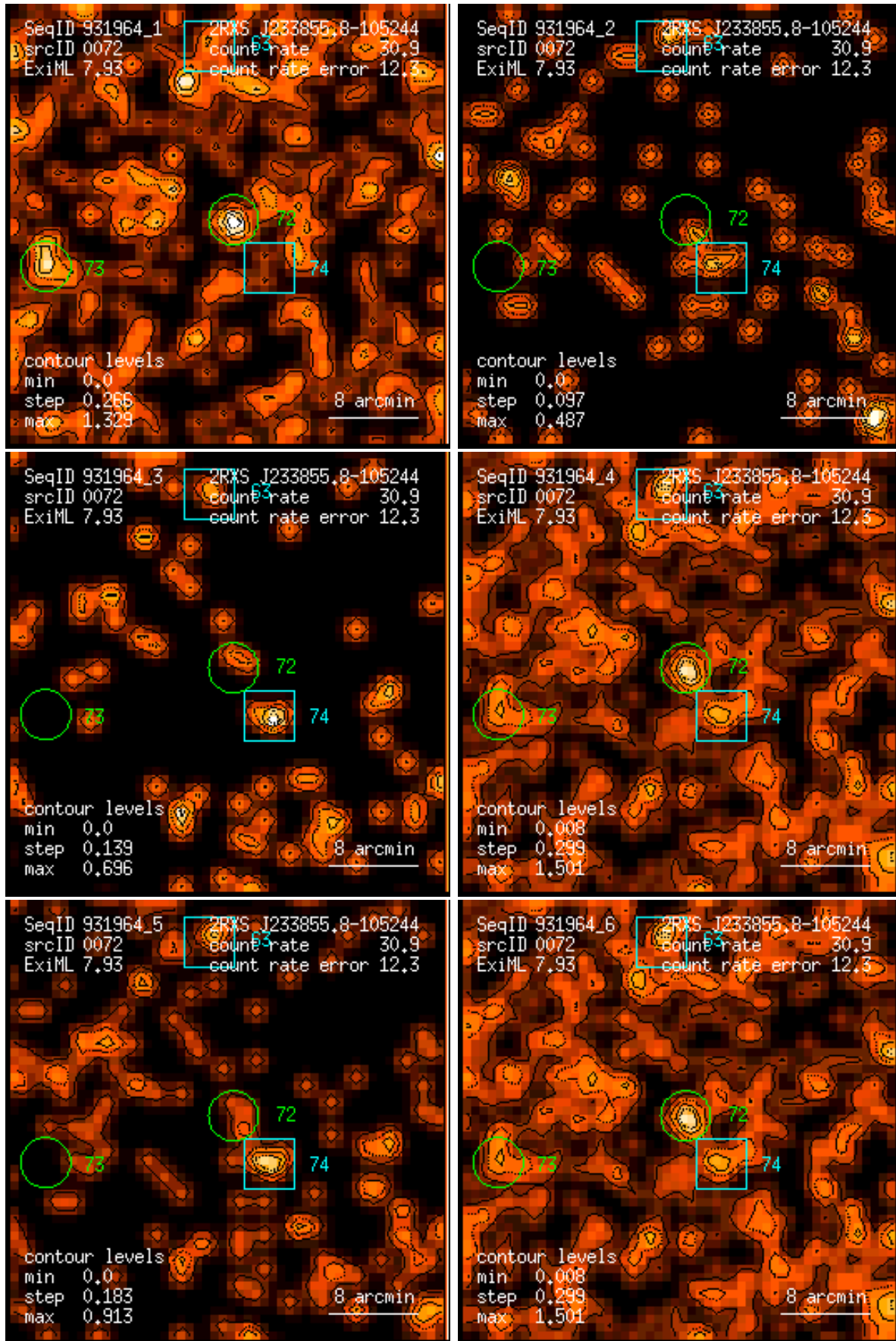
Figure 72: RASS 931964: detection 0072: band rate images, Gaussian filter: (1) PSPC channels 11 – 41, (2) 52 – 90, (3) 91 – 201, (4) 11 – 235, (5) 52 – 201, (6) 11 – 201. Broad band rates in counts/ks. Band rate contour levels in counts/ks/arcmin 2 .
