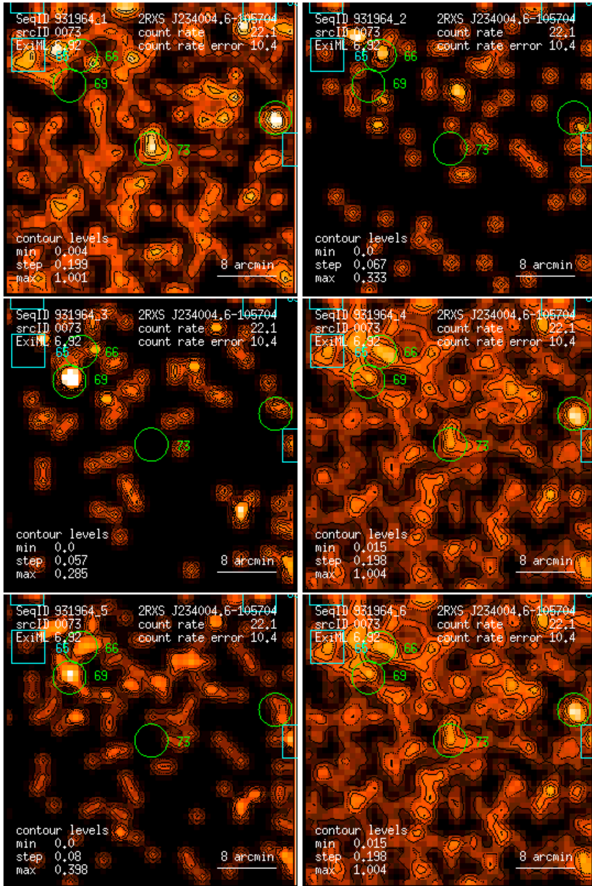
Figure 73: RASS 931964: detection 0073: band rate images, Gaussian filter: (1) PSPC channels 11 – 41, (2) 52 – 90, (3) 91 – 201, (4) 11 – 235, (5) 52 – 201, (6) 11 – 201. Broad band rates in counts/ks. Band rate contour levels in counts/ks/arcmin 2 .
