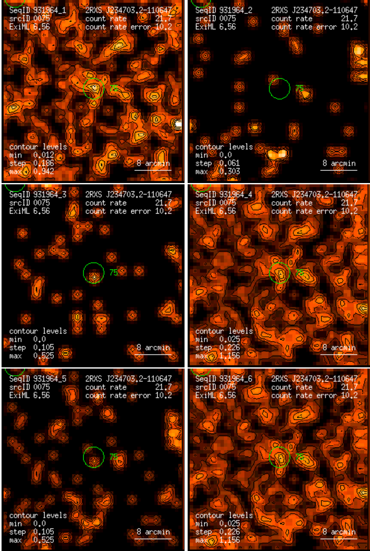
Figure 75: RASS 931964: detection 0075: band rate images, Gaussian filter: (1) PSPC channels 11 – 41, (2) 52 – 90, (3) 91 – 201, (4) 11 – 235, (5) 52 – 201, (6) 11 – 201. Broad band rates in counts/ks. Band rate contour levels in counts/ks/arcmin 2 .
