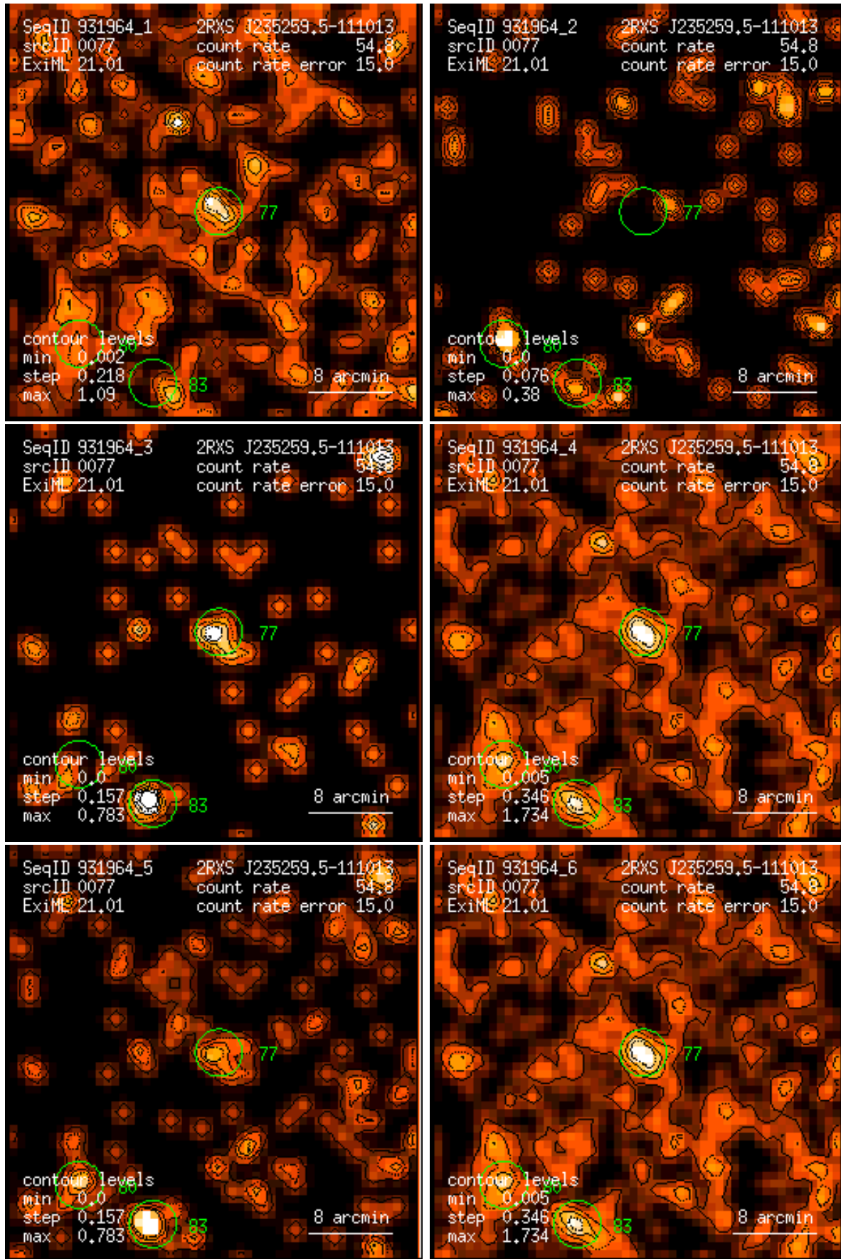
Figure 77: RASS 931964: detection 0077: band rate images, Gaussian filter: (1) PSPC channels 11 – 41, (2) 52 – 90, (3) 91 – 201, (4) 11 – 235, (5) 52 – 201, (6) 11 – 201. Broad band rates in counts/ks. Band rate contour levels in counts/ks/arcmin 2 .
