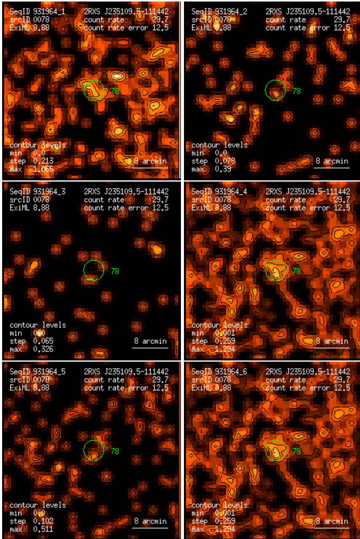
Figure 78: RASS 931964: detection 0078: band rate images, Gaussian filter: (1) PSPC channels 11 – 41, (2) 52 – 90, (3) 91 – 201, (4) 11 – 235, (5) 52 – 201, (6) 11 – 201. Broad band rates in counts/ks. Band rate contour levels in counts/ks/arcmin 2 .
