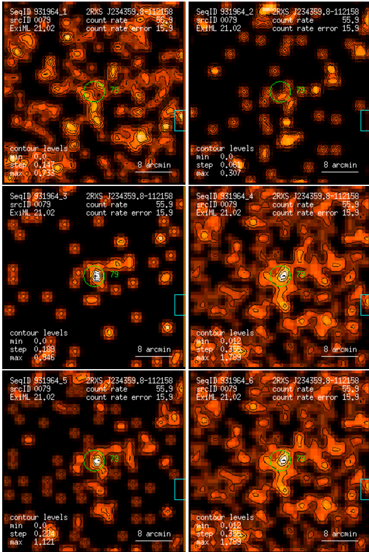
Figure 79: RASS 931964: detection 0079: band rate images, Gaussian filter: (1) PSPC channels 11 – 41, (2) 52 – 90, (3) 91 – 201, (4) 11 – 235, (5) 52 – 201, (6) 11 – 201. Broad band rates in counts/ks. Band rate contour levels in counts/ks/arcmin 2 .
