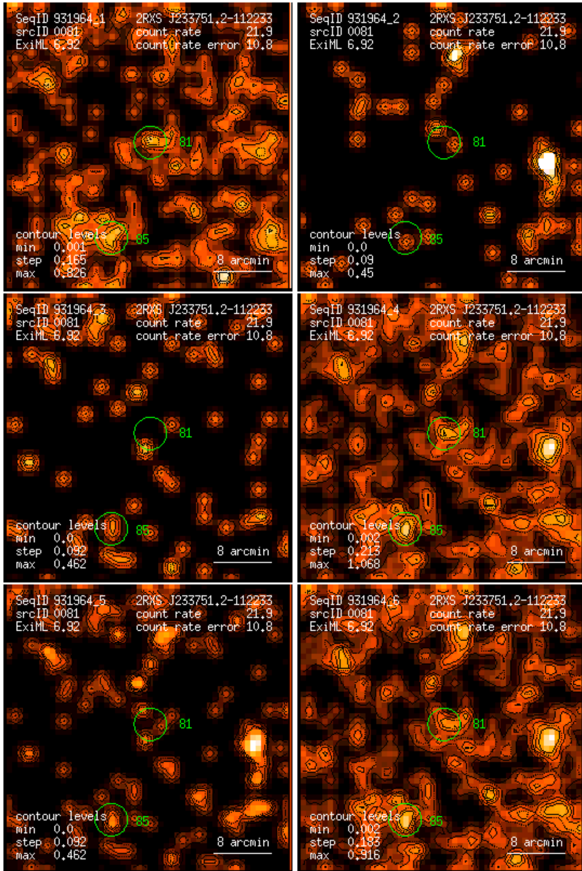
Figure 81: RASS 931964: detection 0081: band rate images, Gaussian filter: (1) PSPC channels 11 – 41, (2) 52 – 90, (3) 91 – 201, (4) 11 – 235, (5) 52 – 201, (6) 11 – 201. Broad band rates in counts/ks. Band rate contour levels in counts/ks/arcmin 2 .
