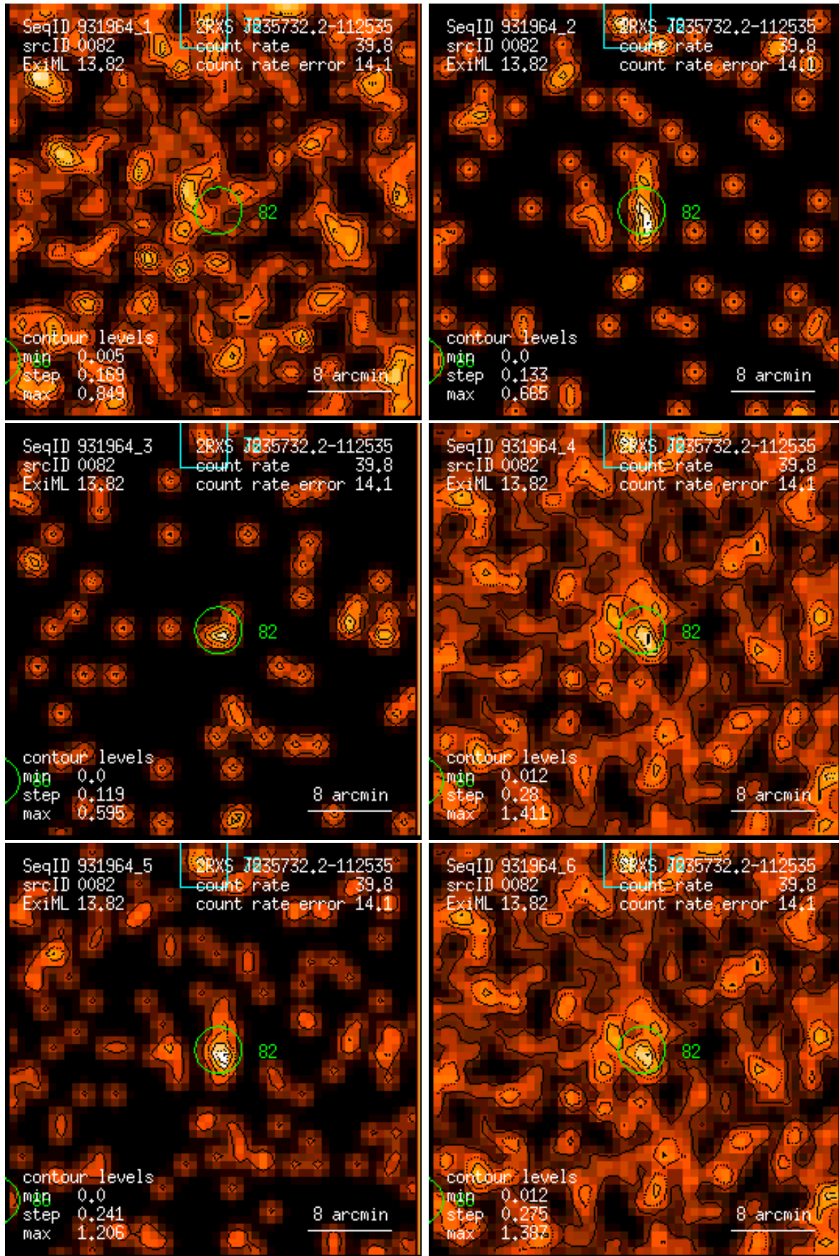
Figure 82: RASS 931964: detection 0082: band rate images, Gaussian filter: (1) PSPC channels 11 – 41, (2) 52 – 90, (3) 91 – 201, (4) 11 – 235, (5) 52 – 201, (6) 11 – 201. Broad band rates in counts/ks. Band rate contour levels in counts/ks/arcmin 2 .
