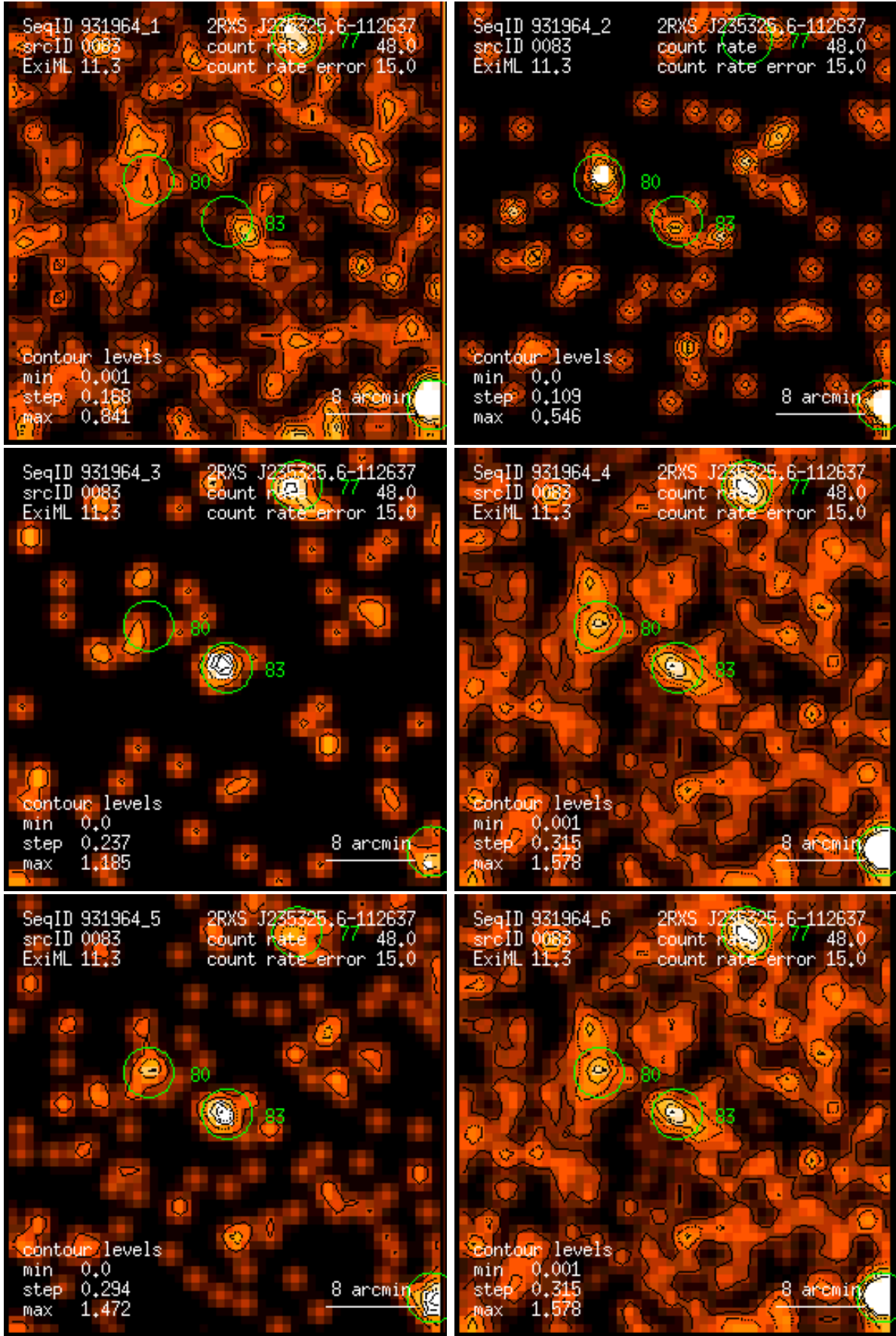
Figure 83: RASS 931964: detection 0083: band rate images, Gaussian filter: (1) PSPC channels 11 – 41, (2) 52 – 90, (3) 91 – 201, (4) 11 – 235, (5) 52 – 201, (6) 11 – 201. Broad band rates in counts/ks. Band rate contour levels in counts/ks/arcmin 2 .
