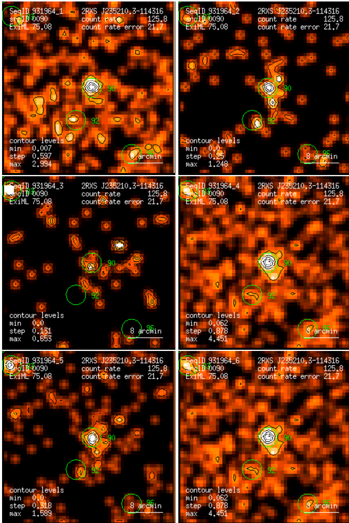
Figure 90: RASS 931964: detection 0090: band rate images, Gaussian filter: (1) PSPC channels 11 – 41, (2) 52 – 90, (3) 91 – 201, (4) 11 – 235, (5) 52 – 201, (6) 11 – 201. Broad band rates in counts/ks. Band rate contour levels in counts/ks/arcmin 2 .
