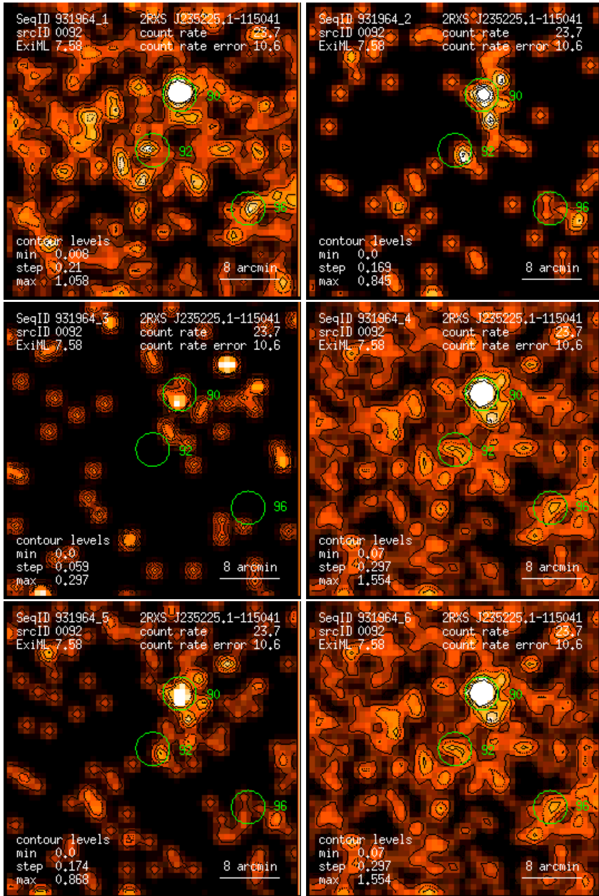
Figure 92: RASS 931964: detection 0092: band rate images, Gaussian filter: (1) PSPC channels 11 – 41, (2) 52 – 90, (3) 91 – 201, (4) 11 – 235, (5) 52 – 201, (6) 11 – 201. Broad band rates in counts/ks. Band rate contour levels in counts/ks/arcmin 2 .
