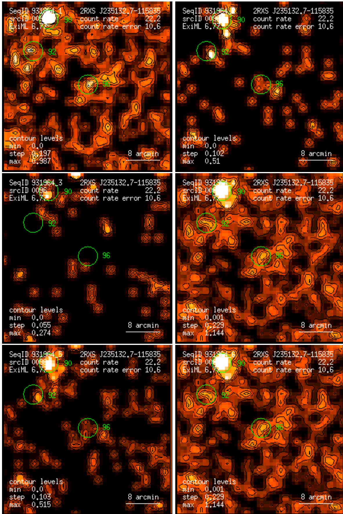
Figure 96: RASS 931964: detection 0096: band rate images, Gaussian filter: (1) PSPC channels 11 – 41, (2) 52 – 90, (3) 91 – 201, (4) 11 – 235, (5) 52 – 201, (6) 11 – 201. Broad band rates in counts/ks. Band rate contour levels in counts/ks/arcmin 2 .
