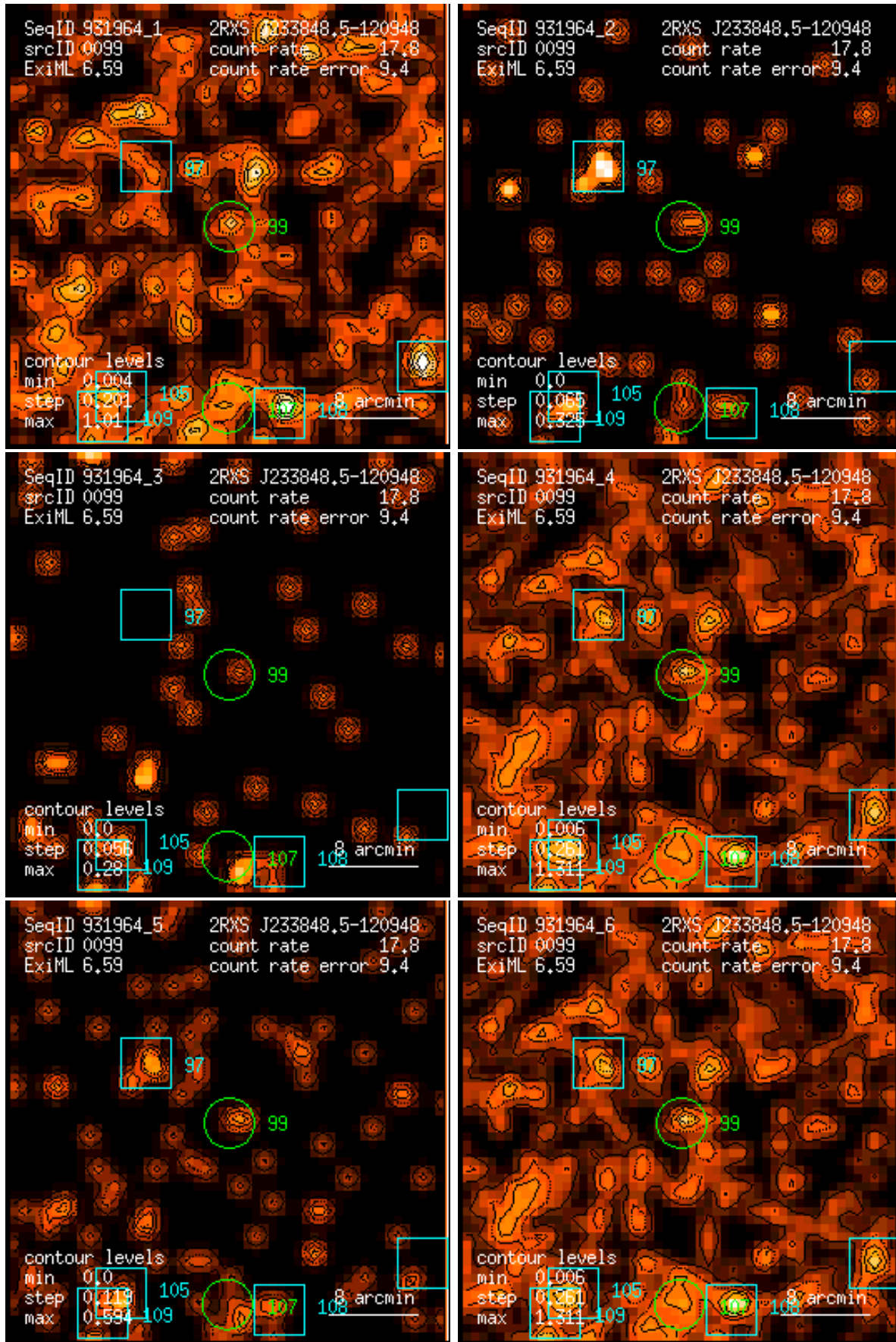
Figure 99: RASS 931964: detection 0099: band rate images, Gaussian filter: (1) PSPC channels 11 – 41, (2) 52 – 90, (3) 91 – 201, (4) 11 – 235, (5) 52 – 201, (6) 11 – 201. Broad band rates in counts/ks. Band rate contour levels in counts/ks/arcmin 2 .
