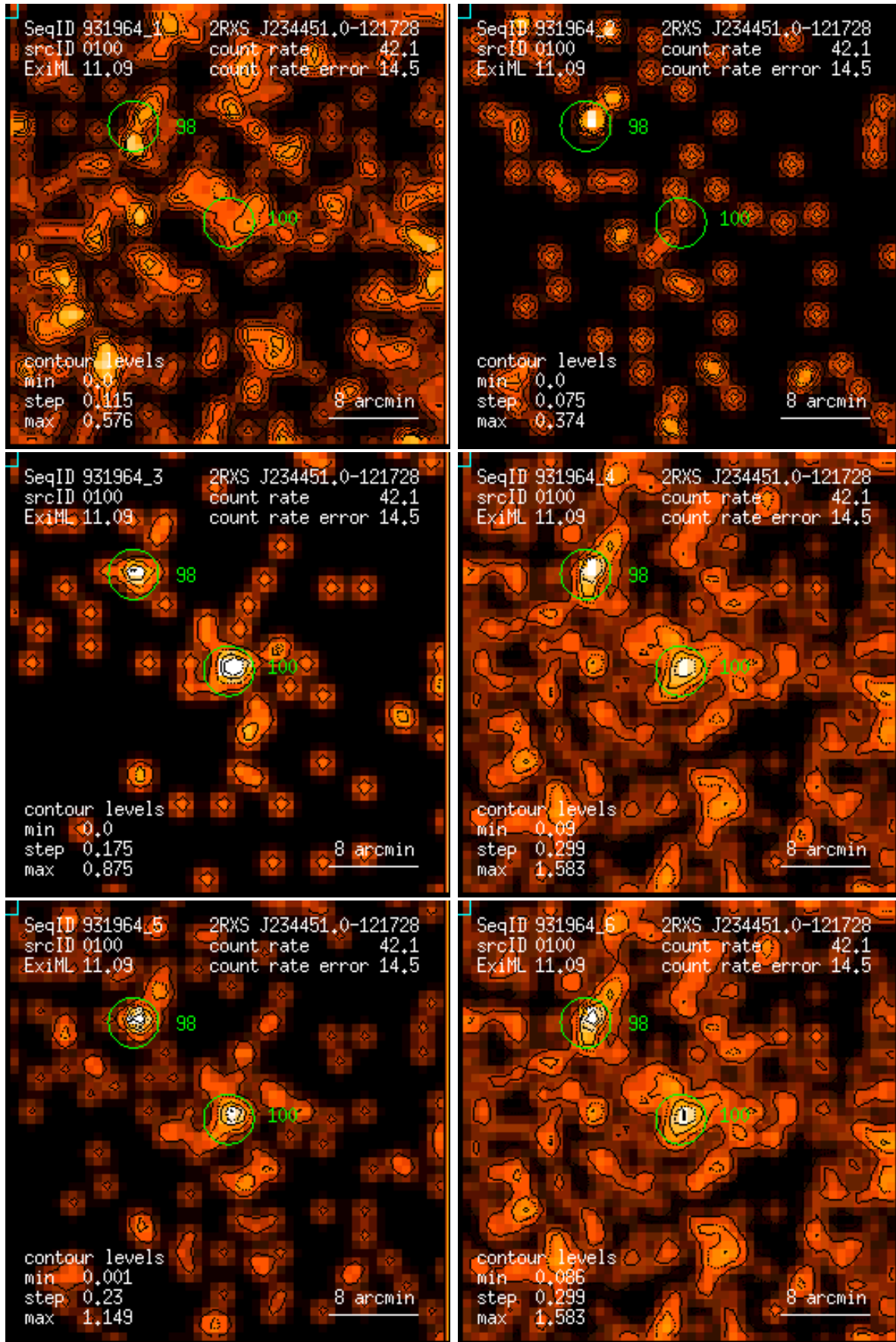
Figure 100: RASS 931964: detection 0100: band rate images, Gaussian filter: (1) PSPC channels 11 – 41, (2) 52 – 90, (3) 91 – 201, (4) 11 – 235, (5) 52 – 201, (6) 11 – 201. Broad band rates in counts/ks. Band rate contour levels in counts/ks/arcmin 2 .
