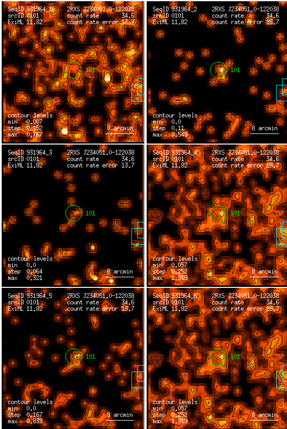
Figure 101: RASS 931964: detection 0101: band rate images, Gaussian filter: (1) PSPC channels 11 – 41, (2) 52 – 90, (3) 91 – 201, (4) 11 – 235, (5) 52 – 201, (6) 11 – 201. Broad band rates in counts/ks. Band rate contour levels in counts/ks/arcmin 2 .
