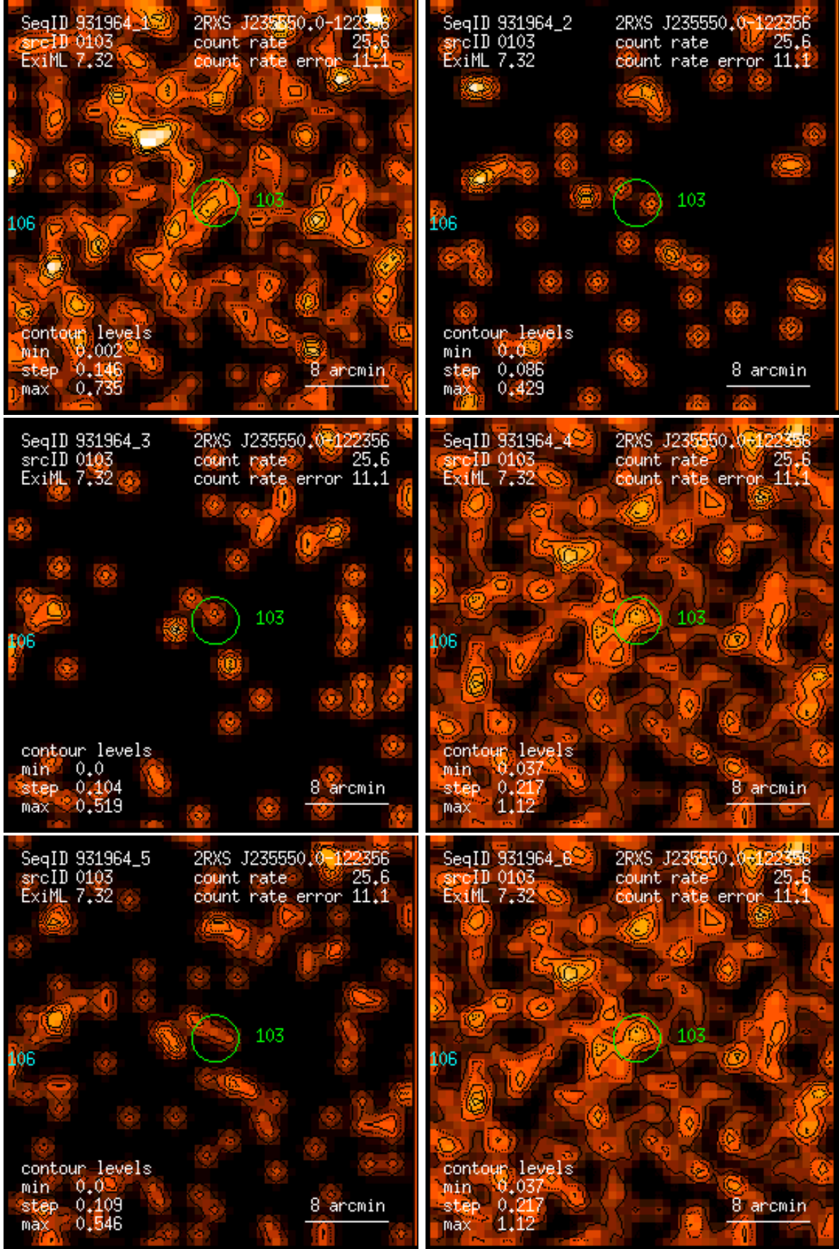
Figure 103: RASS 931964: detection 0103: band rate images, Gaussian filter: (1) PSPC channels 11 – 41, (2) 52 – 90, (3) 91 – 201, (4) 11 – 235, (5) 52 – 201, (6) 11 – 201. Broad band rates in counts/ks. Band rate contour levels in counts/ks/arcmin 2 .
