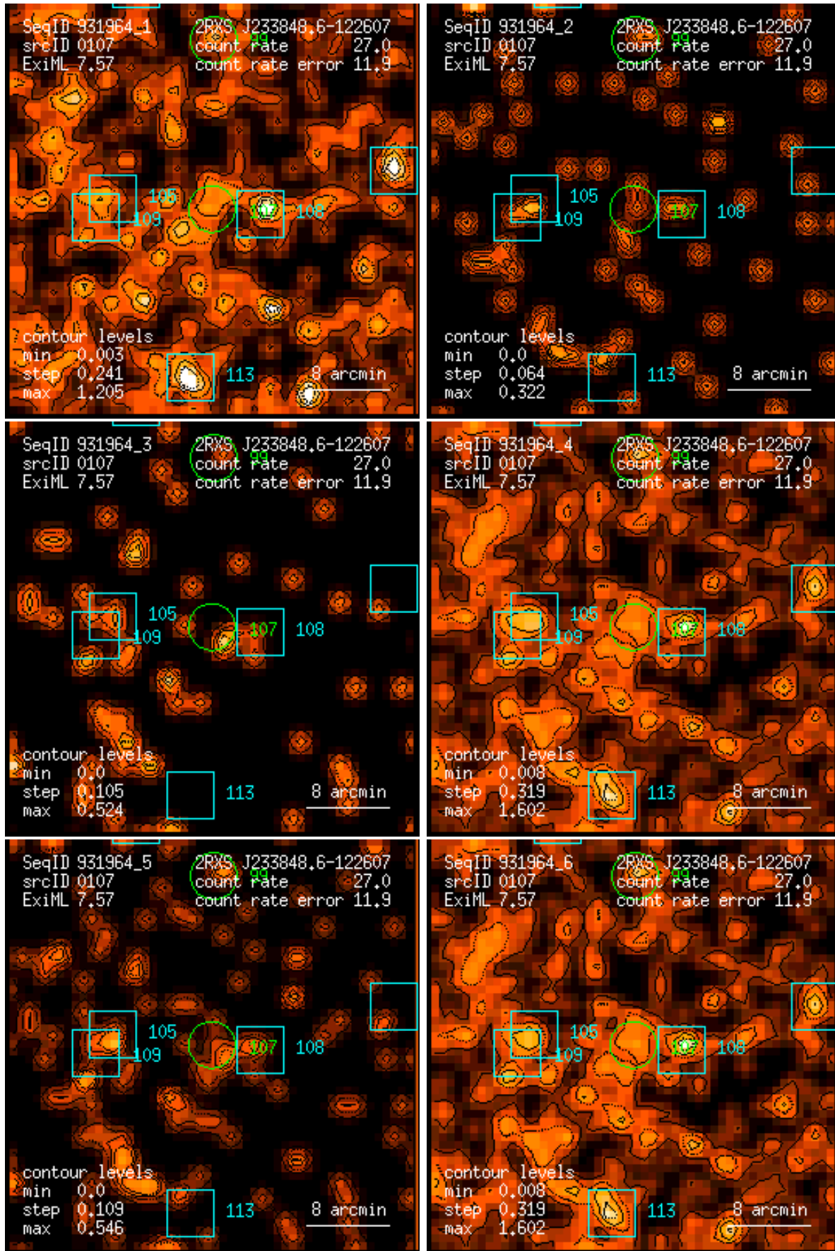
Figure 107: RASS 931964: detection 0107: band rate images, Gaussian filter: (1) PSPC channels 11 – 41, (2) 52 – 90, (3) 91 – 201, (4) 11 – 235, (5) 52 – 201, (6) 11 – 201. Broad band rates in counts/ks. Band rate contour levels in counts/ks/arcmin 2 .
