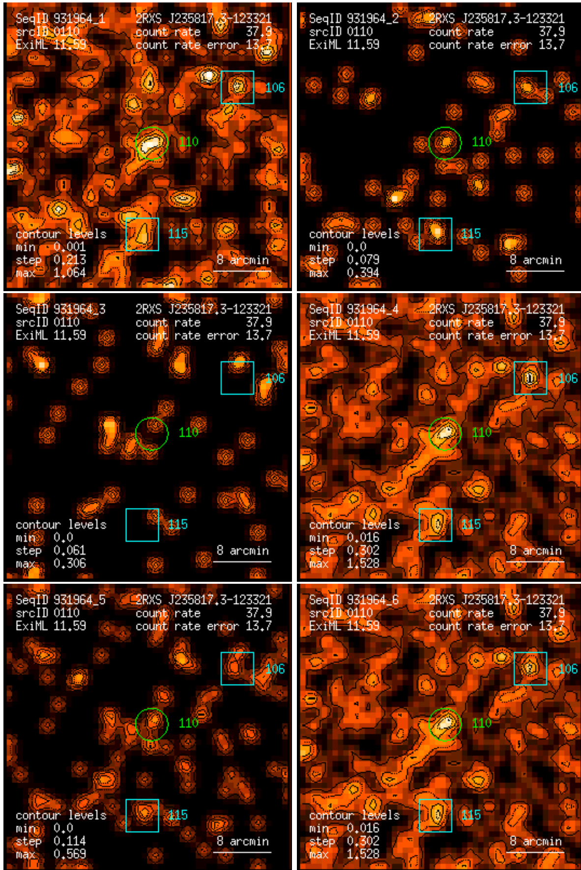
Figure 110: RASS 931964: detection 0110: band rate images, Gaussian filter: (1) PSPC channels 11 – 41, (2) 52 – 90, (3) 91 – 201, (4) 11 – 235, (5) 52 – 201, (6) 11 – 201. Broad band rates in counts/ks. Band rate contour levels in counts/ks/arcmin 2 .
