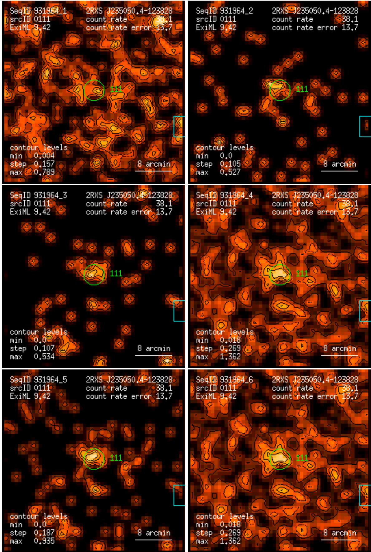
Figure 111: RASS 931964: detection 0111: band rate images, Gaussian filter: (1) PSPC channels 11 – 41, (2) 52 – 90, (3) 91 – 201, (4) 11 – 235, (5) 52 – 201, (6) 11 – 201. Broad band rates in counts/ks. Band rate contour levels in counts/ks/arcmin 2 .
