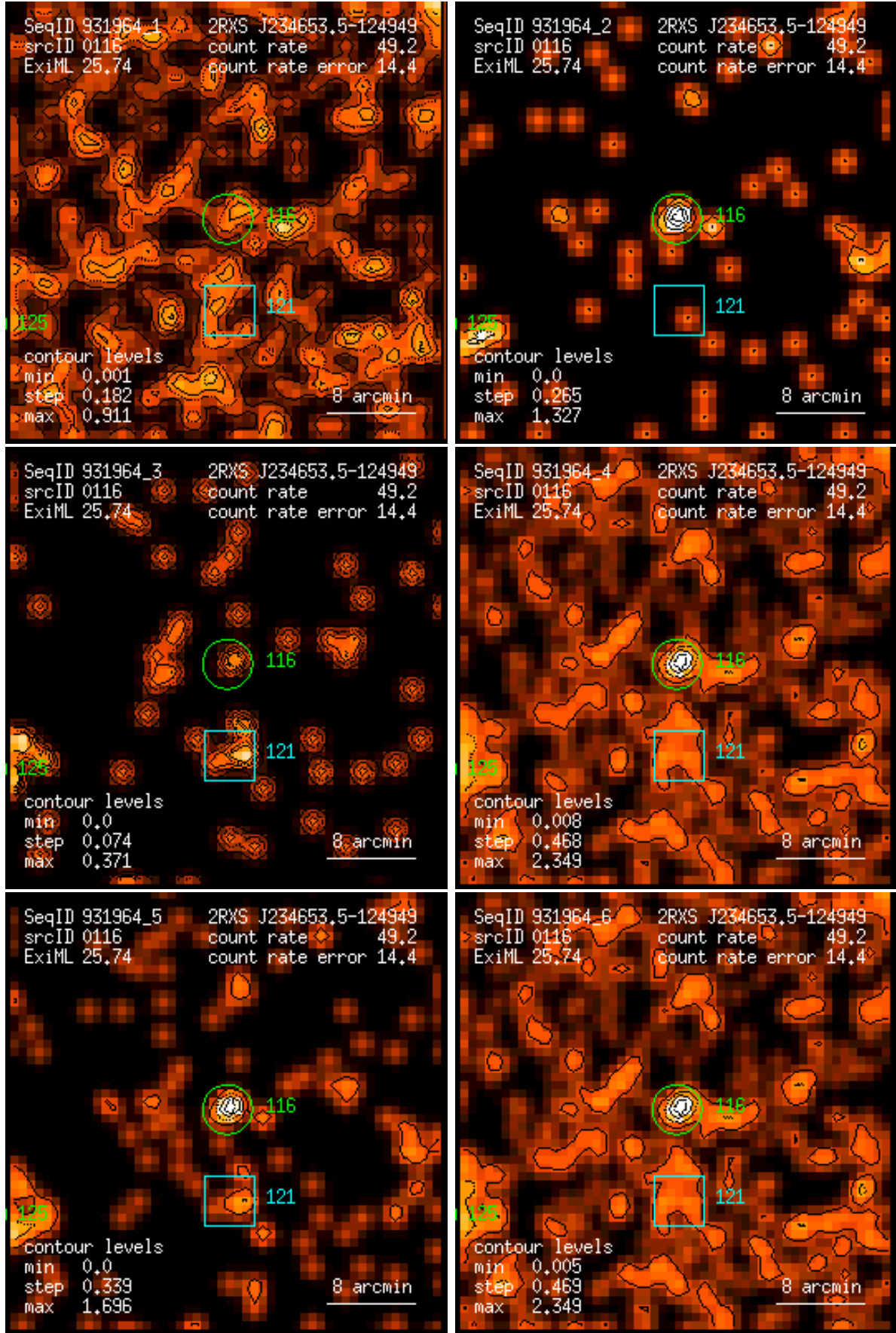
Figure 116: RASS 931964: detection 0116: band rate images, Gaussian filter: (1) PSPC channels 11 – 41, (2) 52 – 90, (3) 91 – 201, (4) 11 – 235, (5) 52 – 201, (6) 11 – 201. Broad band rates in counts/ks. Band rate contour levels in counts/ks/arcmin 2 .
