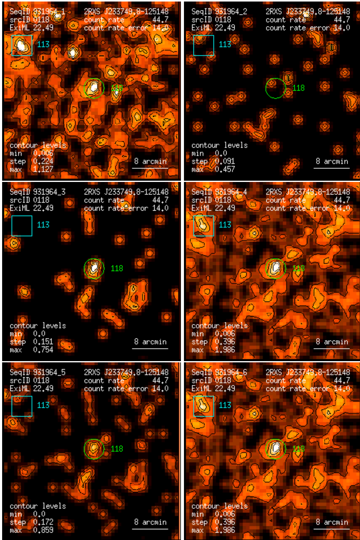
Figure 118: RASS 931964: detection 0118: band rate images, Gaussian filter: (1) PSPC channels 11 – 41, (2) 52 – 90, (3) 91 – 201, (4) 11 – 235, (5) 52 – 201, (6) 11 – 201. Broad band rates in counts/ks. Band rate contour levels in counts/ks/arcmin 2 .
