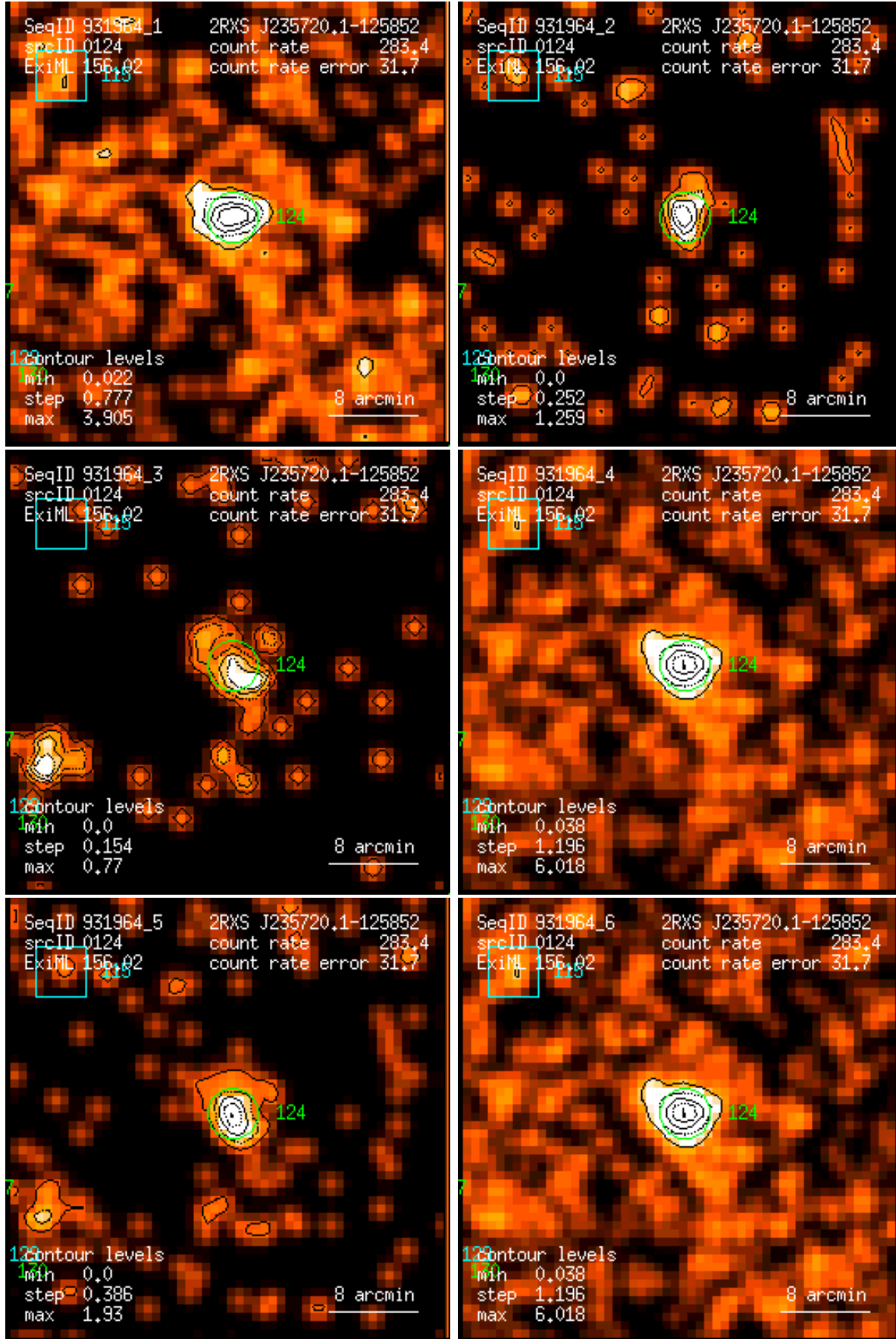
Figure 124: RASS 931964: detection 0124: band rate images, Gaussian filter: (1) PSPC channels 11 – 41, (2) 52 – 90, (3) 91 – 201, (4) 11 – 235, (5) 52 – 201, (6) 11 – 201. Broad band rates in counts/ks. Band rate contour levels in counts/ks/arcmin 2 .
